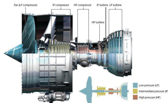
Fig. 2. Three-shaft configuration Trent Family [10]
