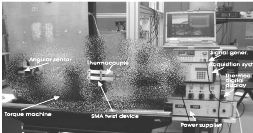
Fig. 20. Experimental setup
