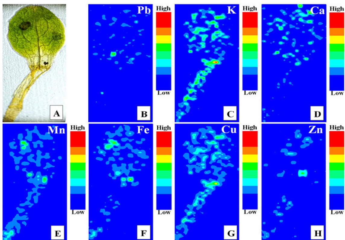
Fig. 6 The \mu -XRF images of Pb, K, Ca, Mn, Fe, Cu, and Zn distribution in longitudinal sections of lettuce seedling in response to a Pb level of 50 \text{ mg kg}^{-1} in studied soil. Samples were collected on the 5th day. Lower fluorescence intensities tend toward the blue end of the color scale while higher intensities tend toward the red end of the color scale.
