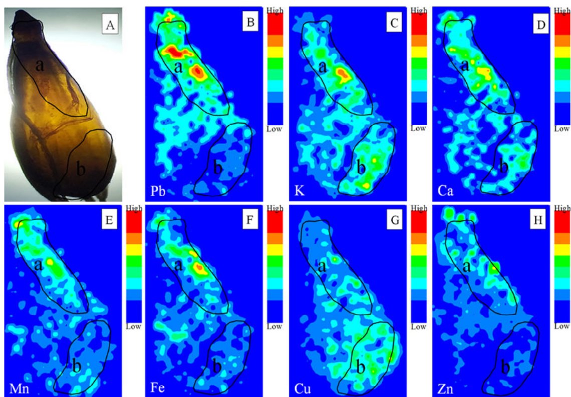
Fig. 4 (A) photo and (B–H) \mu -XRF images of Pb, K, Ca, Mn, Fe, Cu, and Zn distributions in longitudinal sections of dead lettuce seeds (poisoned to death) in response to Pb level of 5000 \text{ mg kg}^{-1} in studied soil. These seeds were collected on the 5th day after sowing. Lower fluorescence intensities (corresponding to lower concentrations) tend toward the blue end of the color scale while higher intensities tend toward the red end of the color scale.
