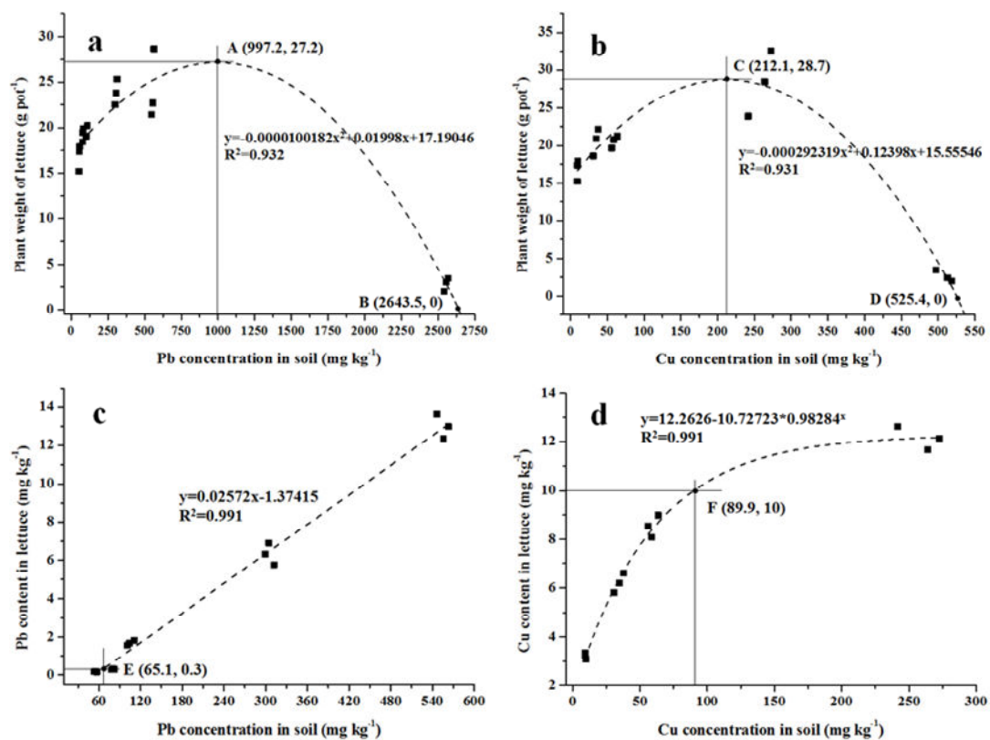
Fig. 2 (a–b) Lettuce plant weight with increasing Pb and Cu levels in contaminated soil, A and B show the yield decreasing concentration and lethal concentration of Pb for lettuce, while C and D show the yield decreasing concentration and lethal concentration of Cu for lettuce. (c–d) The PTE content in lettuce with increasing Pb and Cu concentrations in contaminated soil, E and F show the safety concentrations of Pb and Cu for lettuce.
