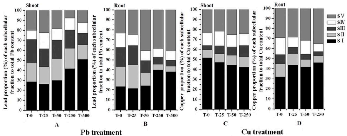
Fig. 3 Subcellular proportions of Pb (A and B) and Cu (C and D) in shoots and roots of lettuce plants under different Pb and Cu levels; SI, SII, SIII, SIV, and SV refer to the supernatant soluble fraction, mitochondrion, nucleus, plastid, and cell wall of lettuce cells, respectively.
