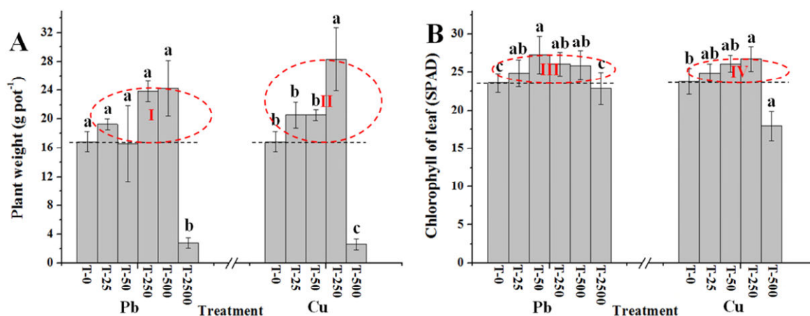
Fig. 1 (A) Weight of lettuce ( Lactuca sativa L.) plants and (B) chlorophyll content of lettuce leaves in studied soils with different Pb and Cu levels; regions “I,” “II,” “III,” and “IV” indicate the area between the value of the control treatment and the highest value, i.e., the hometic effect zone. The T-0, T-25, T-50, T-250, T-500, and T-2500 labels refer to contaminated PTE levels of 0, 25, 50, 250, 500, and 2500 mg kg -1 in soils, respectively. Different lowercase letters on the bar graph indicate significant differences between treatments ( p < 0.05 ).
