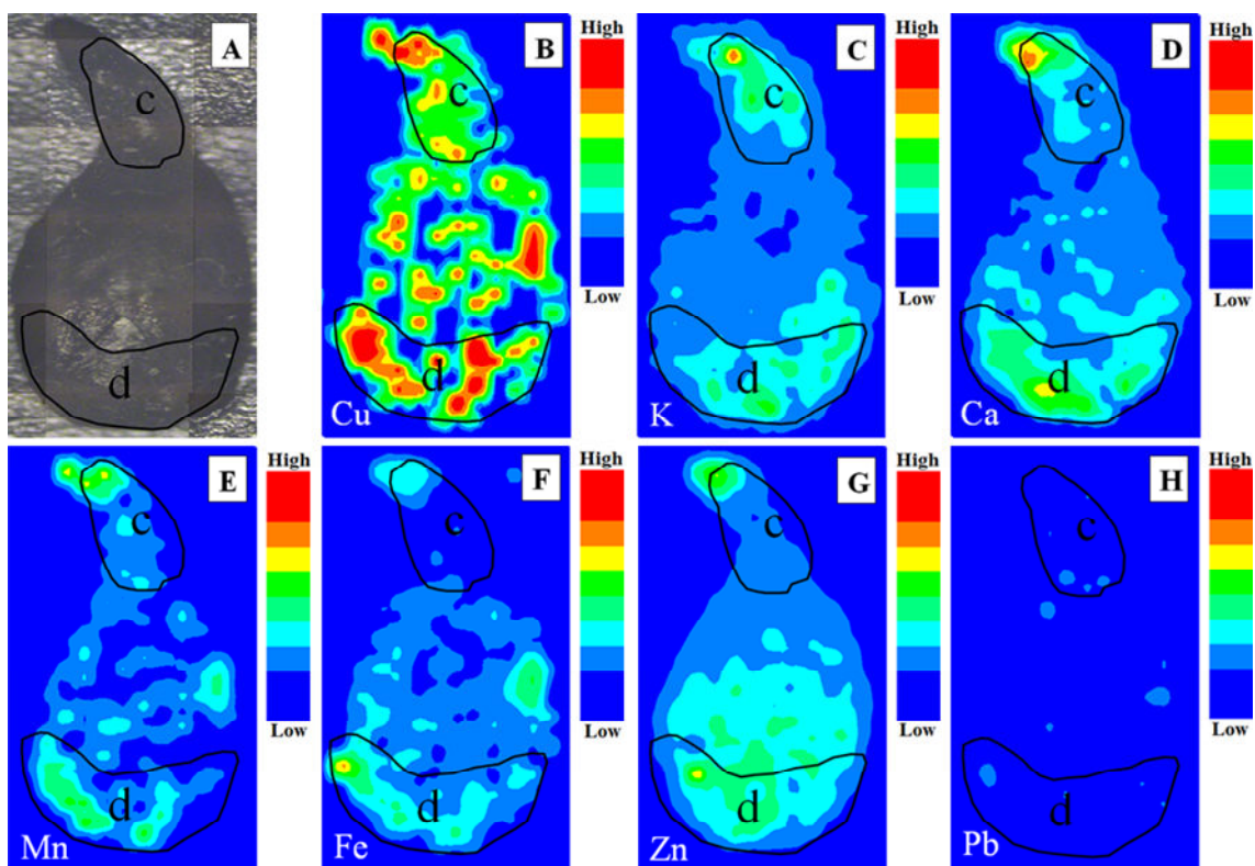
Fig. 5 The \mu -XRF images of Cu, K, Ca, Mn, Fe, Zn, and Pb distribution in longitudinal sections of dead lettuce seeds (poisoned to death) in response to a Cu level of 2500 \text{ mg kg}^{-1} in studied soil. Samples were collected on the 5th day. Higher fluorescence intensities tend toward the red end of the color scale while lower intensities tend toward the blue.
