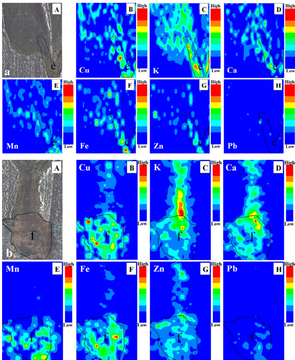
Fig. 7 The \mu -XRF images of Cu, K, Ca, Mn, Fe, Zn, and Pb distribution in longitudinal sections of lettuce seedling (a) shoots and (b) roots in response to Cu levels of 50 \text{ mg kg}^{-1} in studied soil. Samples were collected on the 5th day after sowing. Higher fluorescence intensities (corresponding to higher concentrations) tend toward the red end of the color scale while lower intensities tend toward the blue.
