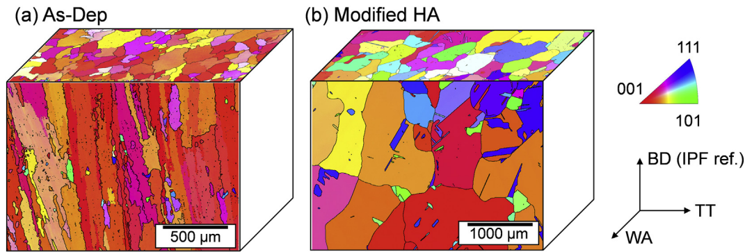
Fig. 11. Inverse pole figure EBSD maps of (a) As-Dep and (b) Modified HA materials, with IPF colouring reference in BD showing high angle ( >15^\circ ) grain boundaries.
