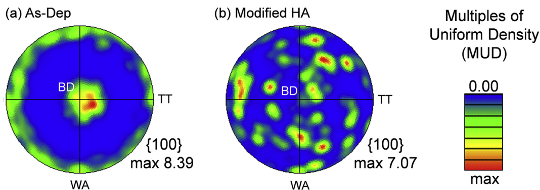
Fig. 12. Pole figures of (a) As-Dep and (b) Modified HA materials, determined from EBSD.
