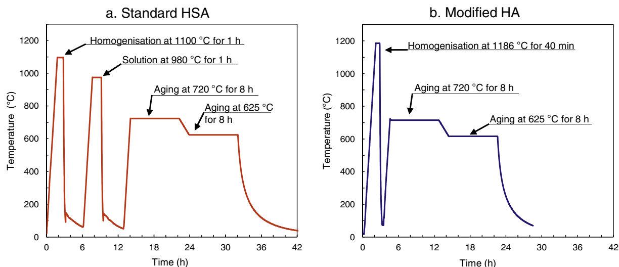
Fig. 4. Measured temperature traces for (a) standard homogenised and solution-aged and (b) modified homogenised and aged WAAM IN718 materials.
