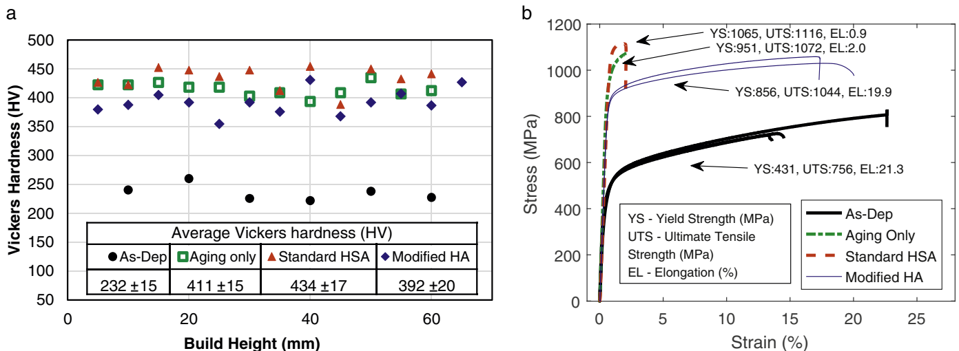
Fig. 10. (a) Vickers hardness with increasing build height and a summary of the average and standard deviation, and (b) engineering stress-strain curves from samples loaded in the build direction at room temperature.
