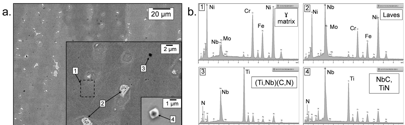
Fig. 8. As-Dep WAAM Inconel 718 material (a) backscatter electron images and (b) corresponding EDX spectra of spot analysis.
