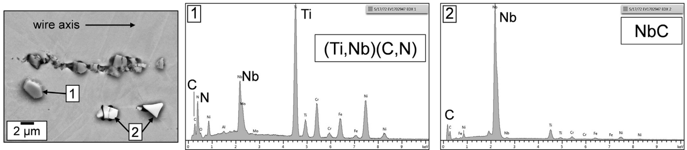
Fig. 5. SEM backscatter electron image and corresponding EDX spectra showing TiN and NbC particles in the wire feedstock.
