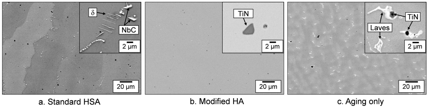
Fig. 9. Backscatter electron images of WAAM IN718 after (a) Standard HSA, (b) Modified HA and (c) Aging only heat treatments.
