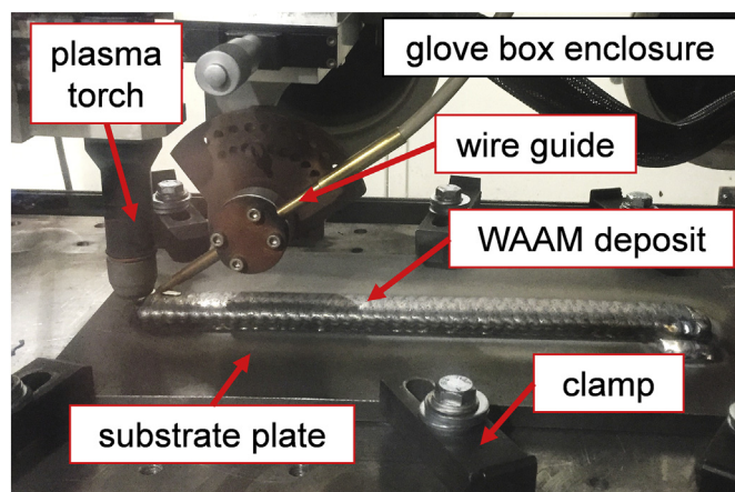
Fig. 1. WAAM equipment setup within the glove box.
