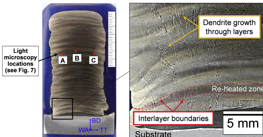
Fig. 6. Macrograph showing locations of light micrographs A, B, C in Fig. 7, dendritic features, re-heated zone and interlayer boundaries.
