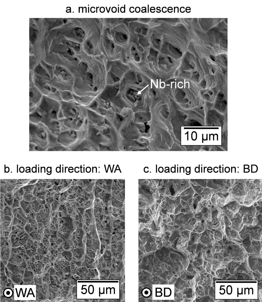
Fig. 15. Secondary electron images of fracture surfaces from tested tensile specimens (stress strain curves in Fig. 13), showing (a) dimples indicating microvoid coalescence characteristic of ductile fracture, and differences in dimple patterns observed in fracture surfaces normal to (b) wall axis and (c) build directions.
