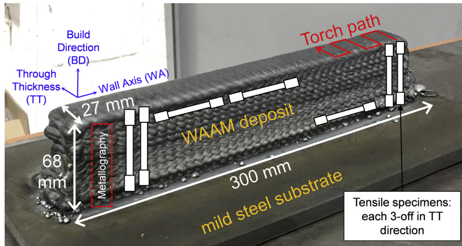
Fig. 2. Photograph of IN718 WAAM wall labelled with build dimensions, direction axes, oscillating torch path and extraction locations of metallographic slice and tensile specimens.
