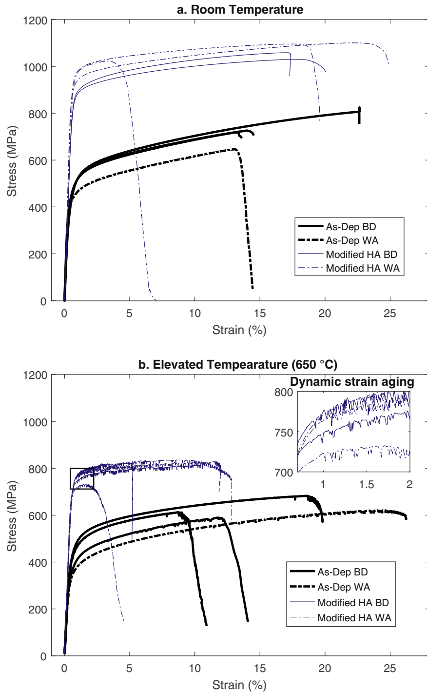
Fig. 13. Engineering stress-strain curves of As-Dip and Modified HA tensile specimens loaded separately in the build and wall axis directions (BD and WA respectively), at (a) room and (b) elevated temperature (650 °C).
