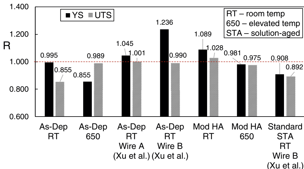
Fig. 14. Property ratios for yield strength (YS) and ultimate tensile strength (UTS) of WAAM IN718 materials from this work and reported values from Xu et al. [10].
