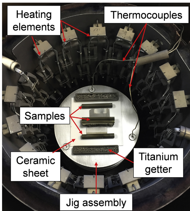
Fig. 3. Internal chamber of vacuum furnace used to perform heat treatments.
