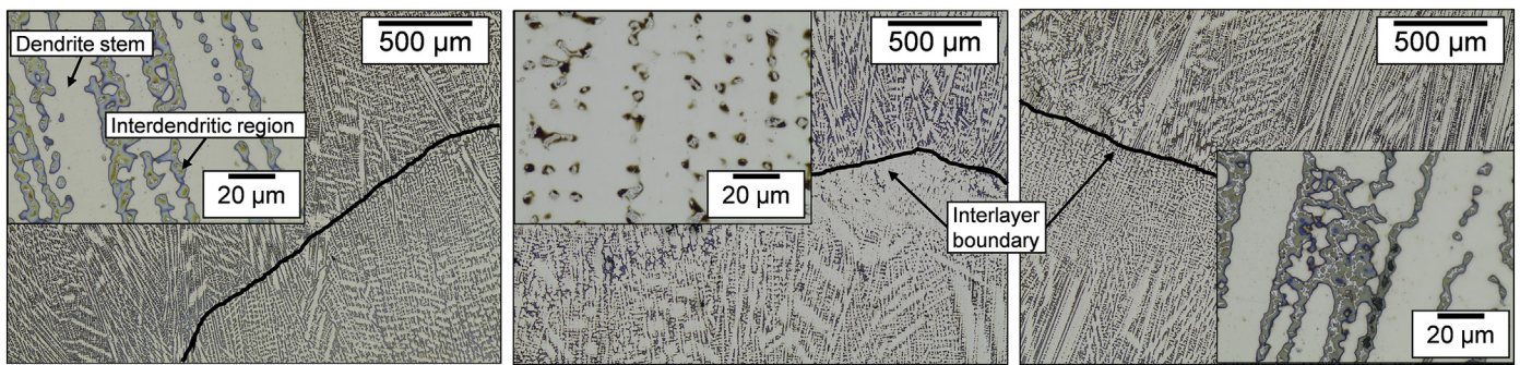
Fig. 7. Optical micrographs of As-Dep WAAM Inconel 718 material in the through-thickness section at locations shown in Fig. 6.
