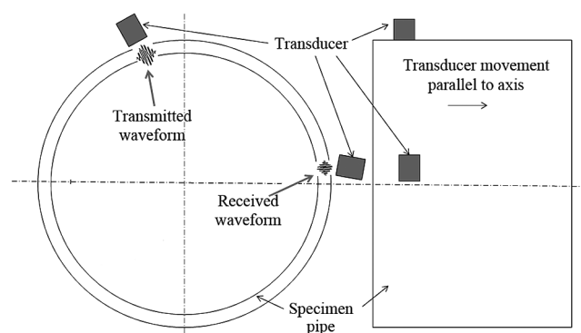
Figure 11. Scanning direction during radial measurements; transducer arrangement moves axially and the pipe is stationary
