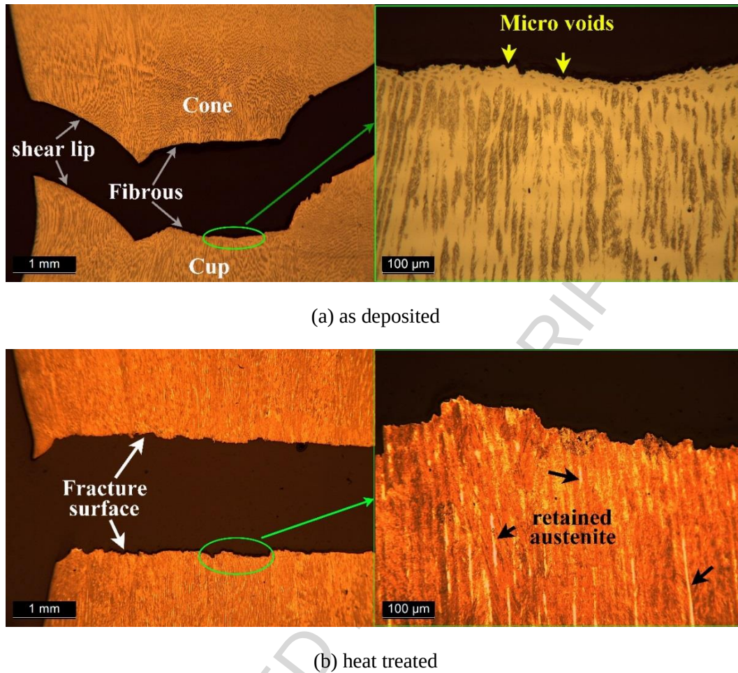
Fig. 12 Optical microscopy of the joint fracture surface (longitudinal section)
