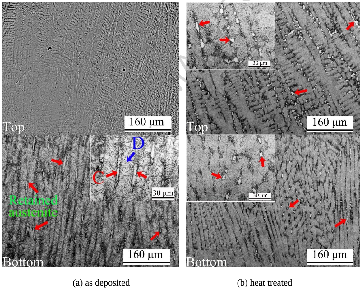
Fig. 3 Microstructure of the maraging steel produced by WAAM process
