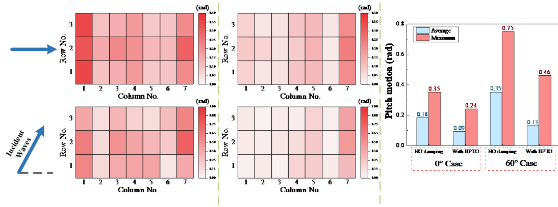
(a) Pitch motion
