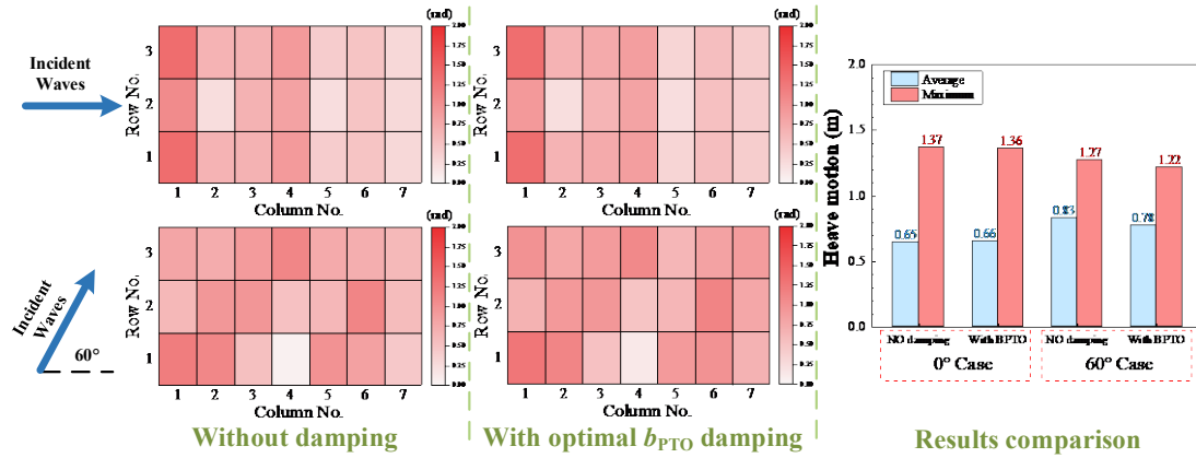
(b) Heave motion
