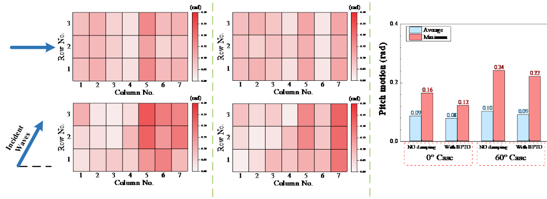
Figure 18 Impact of optimal b_{PTO} damping on the motion response of the array at T=5.3 s
