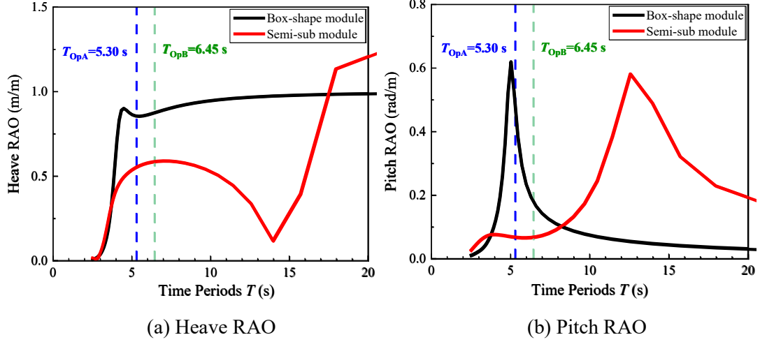
Figure 2 Motion response RAOs between Box-type and Semi-submersible floating modules
