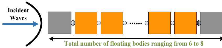
Figure 10 Top view sketch of a row of FPV array
