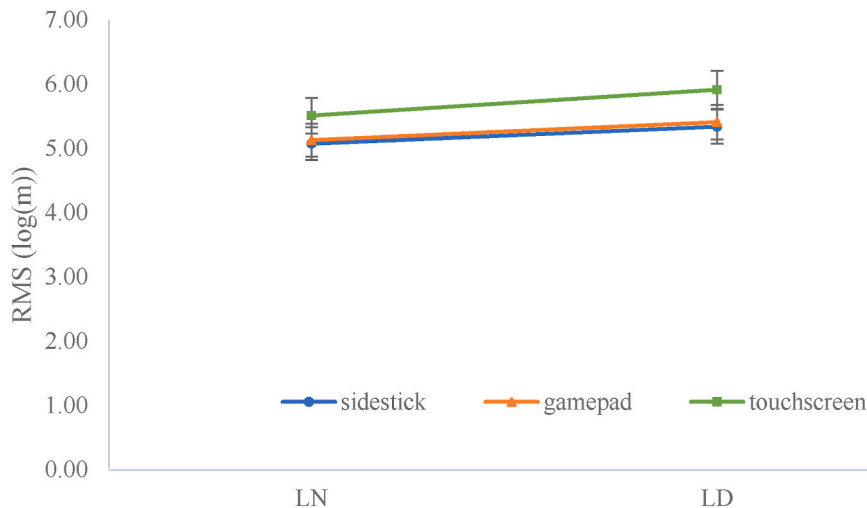
Fig. 5. Participants' flight path deviation (in log(m)) while interacting with three different types of inceptors in landing with disturbance (LD) and landing with non-disturbance (LN) scenarios. Mean and 95% confidence intervals.
