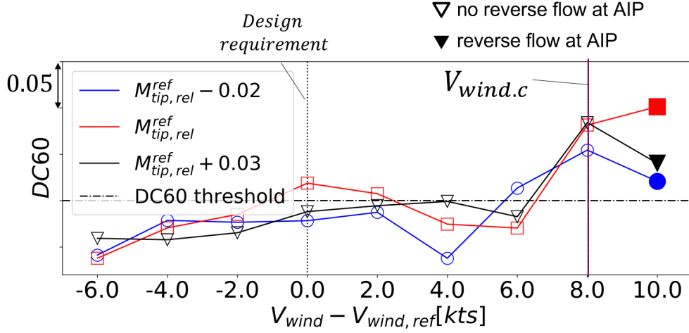
Figure 4: Effect of fan rotational speed on DC60 at the AIP. The intake threshold crosswind velocity ( V_{wind,c} ) was determined based on no separation at the AIP. Steady RANS-IBMSG analyses, counter-rotating configuration
