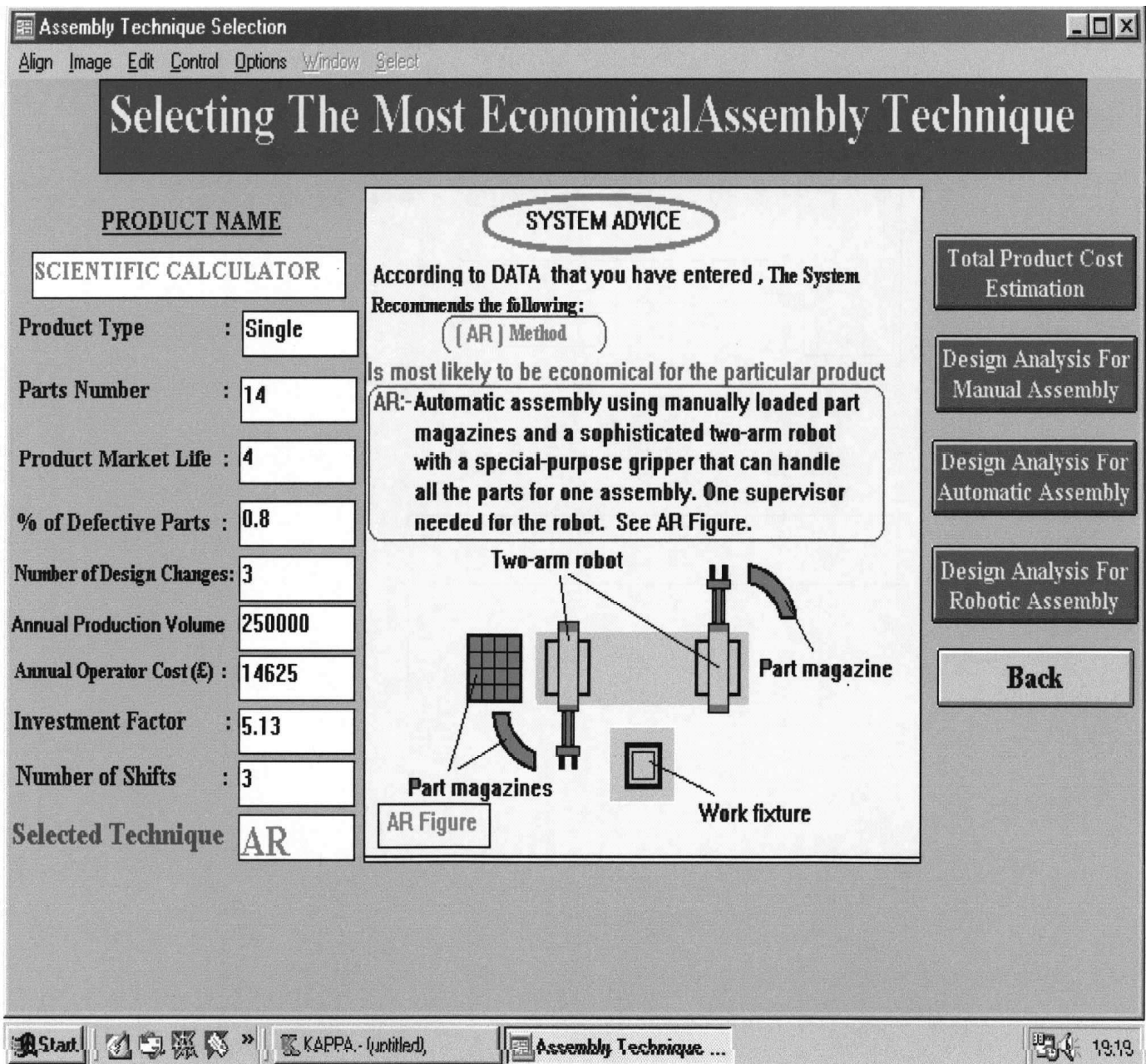
Fig. 12 System window of the appropriate assembly selection for the scientific calculator
