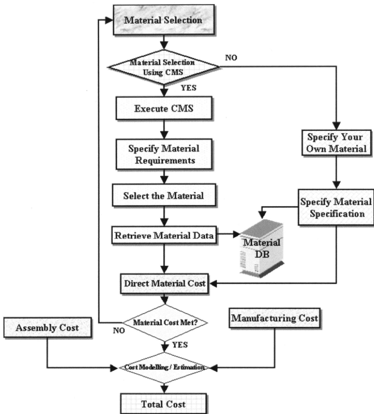
Fig. 2 Material selection/costing module
