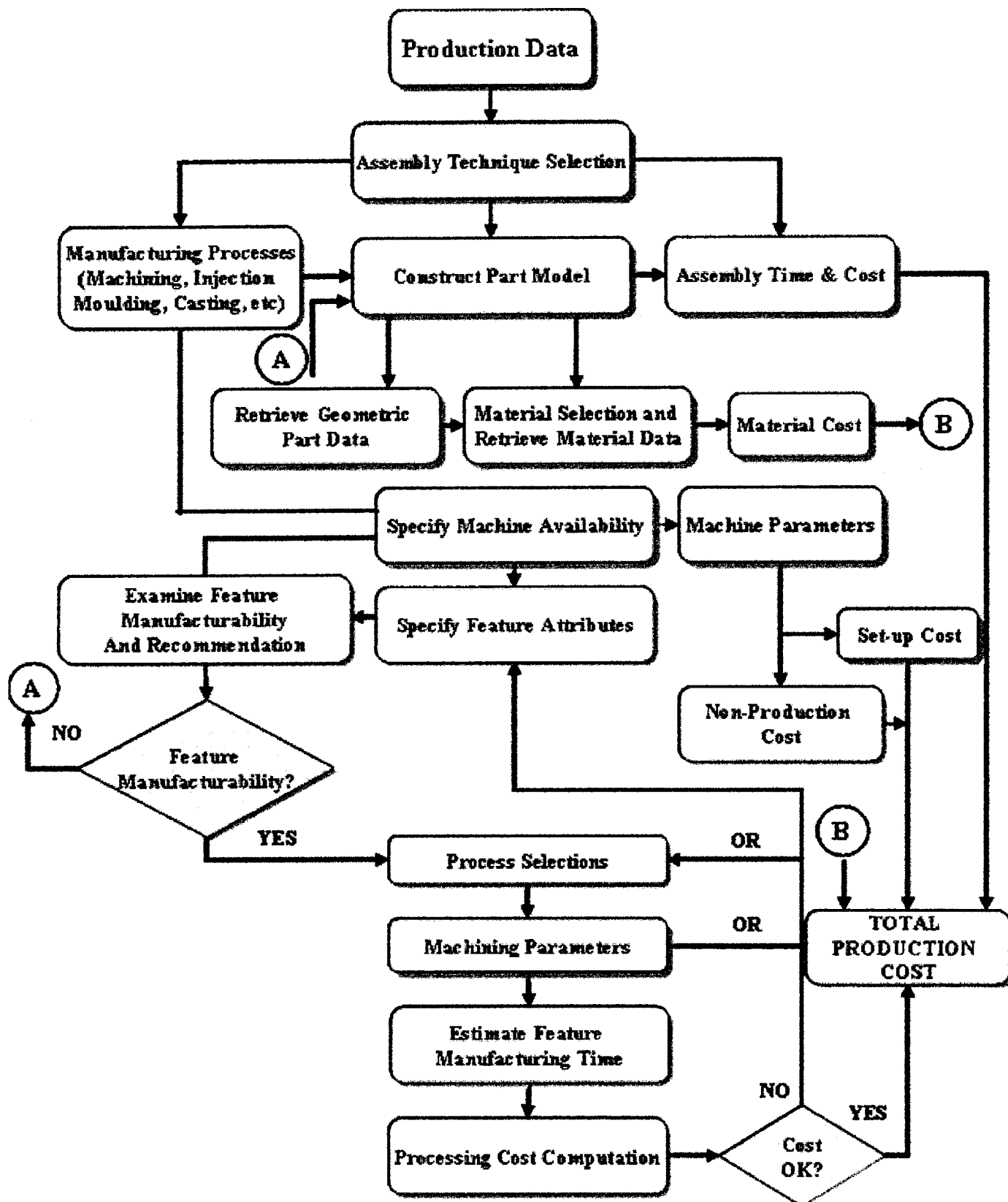
Fig. 10 System scenario for the machined component cost analysis process
