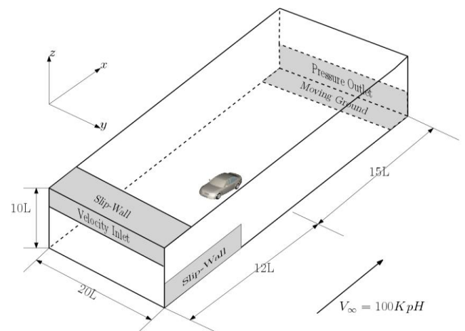
Figure 5 Computational Domain and Boundary Conditions.
