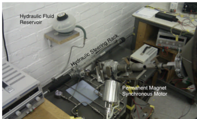
Figure A1. EPAS experimental apparatus (left)
