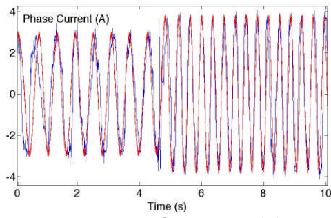
Figure 13e. 3A-4A motor phase current (A)
