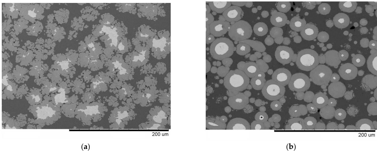
Figure 5. Microstructure of composites: IV (a) and V (b). Designation of composites is given in Table 1.
