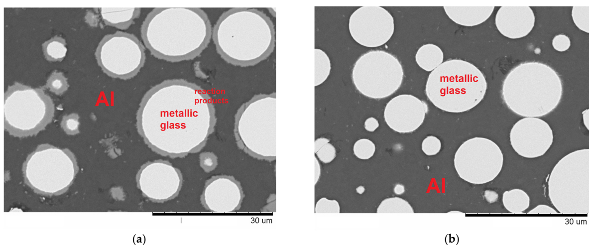
Figure 3. Micrographs of composites sintered from the \text{Al} + 20 \text{ vol.}\% \text{ Fe}_{66}\text{Cr}_{10}\text{Nb}_5\text{B}_{19} powder mixture at 570^\circ\text{C} , 1 min: (a) 40 MPa, (b) 80 MPa. The interfacial reactions were hindered during spark plasma sintering at 80 MPa.
