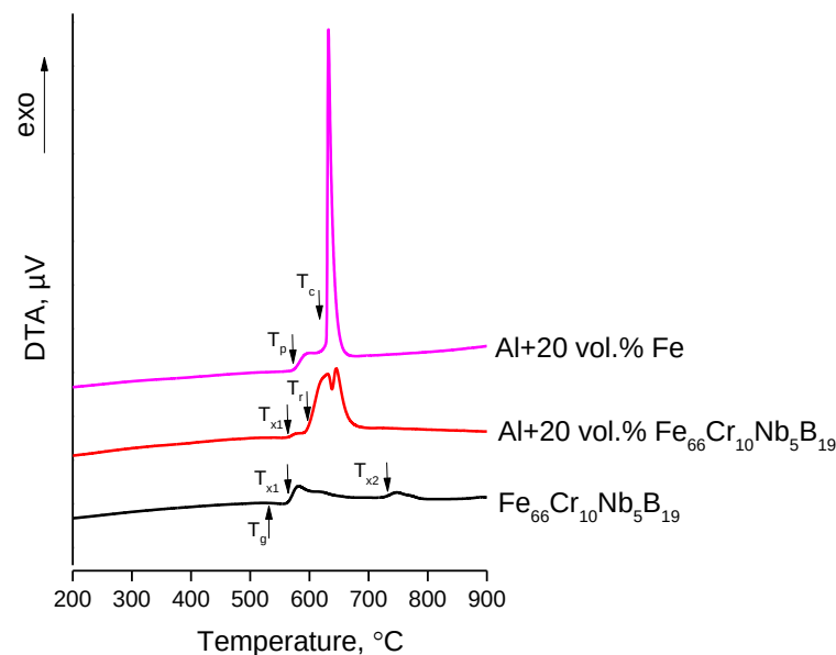
Figure 4. Differential thermal calorimetry traces of the pre-pressed Al + 20 vol.% Fe and Al + 20 vol.% \text{Fe}_{66}\text{Cr}_{10}\text{Nb}_5\text{B}_{19} mixtures and the as-atomized \text{Fe}_{66}\text{Cr}_{10}\text{Nb}_5\text{B}_{19} glassy powder. The characteristic temperatures of the thermal events are marked by arrows: glass transition T_g and crystallization onset temperatures T_{x1} and T_{x2} of the \text{Fe}_{66}\text{Cr}_{10}\text{Nb}_5\text{B}_{19} glass, the onset temperature of reaction between the \text{Fe}_{66}\text{Cr}_{10}\text{Nb}_5\text{B}_{19} glass and aluminum T_r , pre-combustion temperature T_c and combustion temperature of the Al + 20 vol.% Fe mixture.
