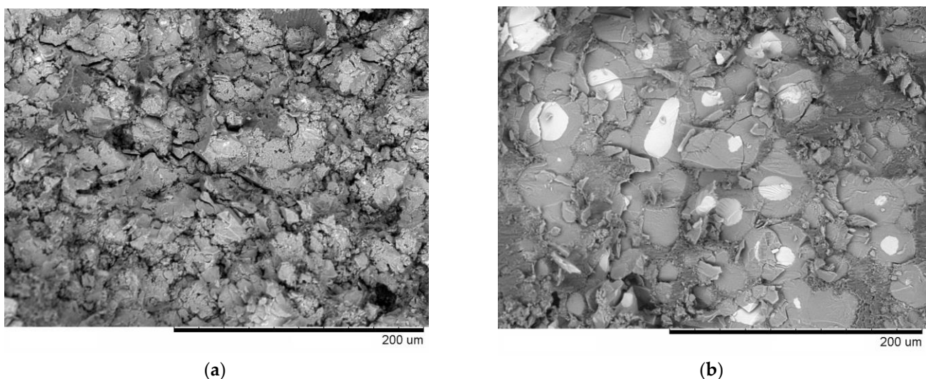
Figure 7. Fracture surface of samples tested under compression: composite IV (a) and composite V (b). Designation of composites is given in Table 1.
