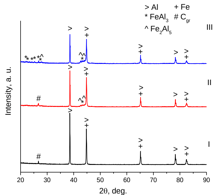
Figure 2. XRD patterns of composites I, II and III. The presence of graphite (002) reflection at 2\theta = 26.6^\circ is due to the presence of the residual graphite foil adhered to the specimen. Designation of composites is given in Table 1.
