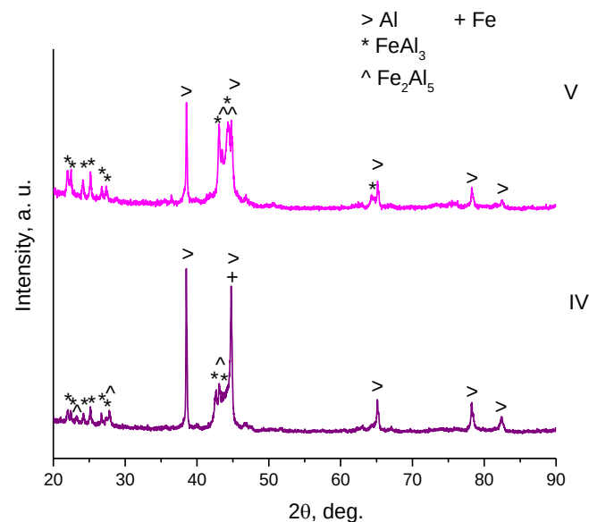
Figure 6. XRD patterns of composites IV and V. Designation of composites is given in Table 1.
