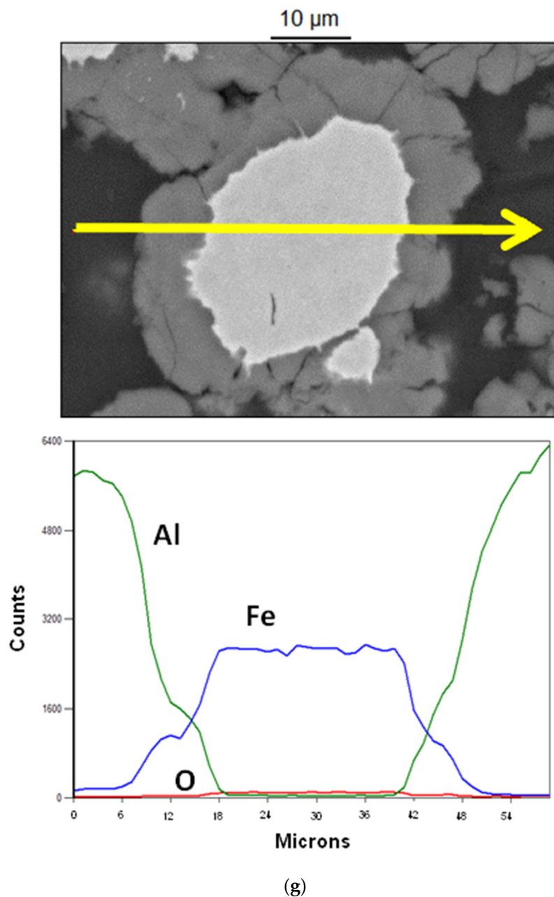
Figure 1. Microstructure of composites derived from the Al + 20 vol.% Fe mixture: I (a,b), II (c,d) and III (e,f). The energy dispersive spectroscopy data for composite III: a core-shell particle is analyzed (g). Designation of composites is given in Table 1.
