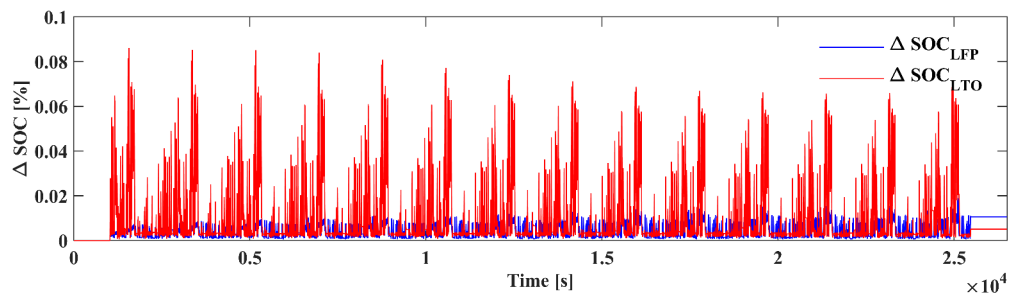
Fig. 9. The difference between the maximum and minimum SOC of modules in the LFP and LTO battery sub-packs
