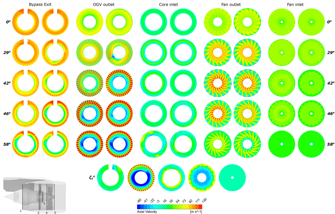
Fig. 7 Internal flow field development for the complete VPF hysteresis loop using axial velocity contours at five different locations inside the engine for the complete VPF hysteresis loop. The forward-to-reverse thrust operation is represented by the left column at each engine station and the right column shows the reverse-to-forward thrust operation. Core inlet plane is scaled for a more detailed view.
