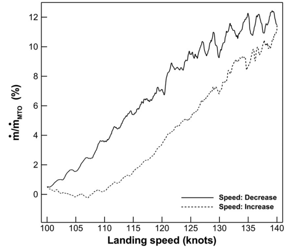
Fig. 15 Aircraft landing speed hysteresis loop: Percentage of mass flowrate evolution ingested by the engine and normalized by the corresponding maximum takeoff value
