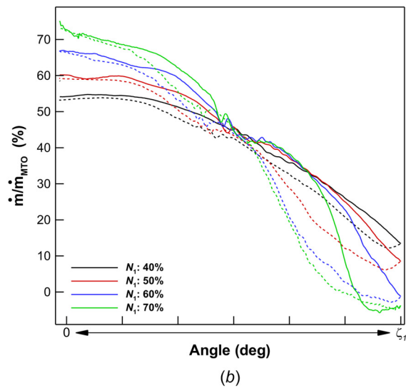
Fig. 12 Effect of fan rotational speed on the VPF hysteresis loop: Fig. 12(a) shows the mass flow rate percentage evolution over time while Fig. 12(b) shows the VPF hysteresis loops. The forward-to-reverse thrust operations are depicted by solid lines while dashed lines represent the reverse-to-forward thrust operations.
