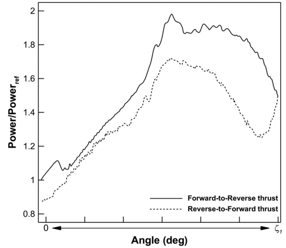
Fig. 9 Fan power absorption evolution normalized by the nominal forward flow power for the complete VPF hysteresis loop
