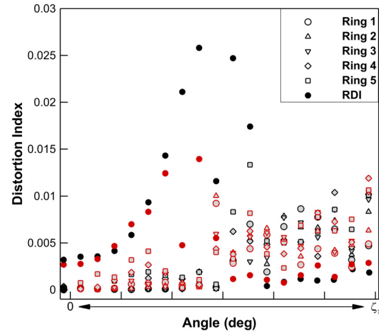
Fig. 11 CDI and RDI core distortion levels for the complete VPF hysteresis loop
