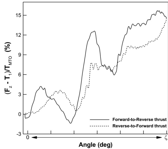
Fig. 10 Percentage of axial decelerating force evolution normalized by the maximum takeoff value for the complete VPF hysteresis loop
