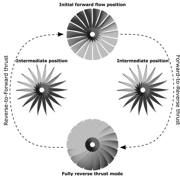
Fig. 2 VPF blade airfoils transition from forward flow position to the reverse thrust mode setting and back showing the complete VPF hysteresis loop
