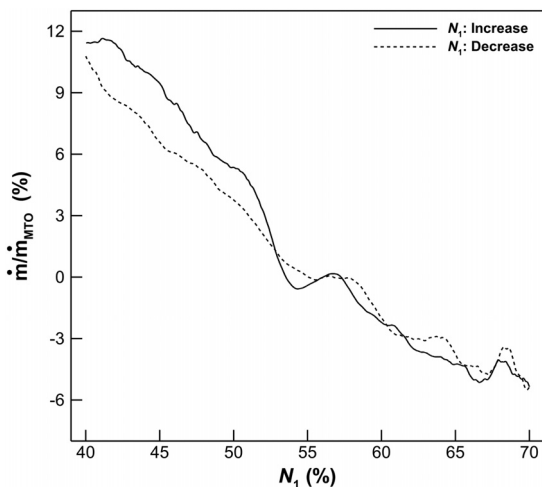
Fig. 14 Fan rotational speed hysteresis loop: Percentage of mass flowrate evolution ingested by the engine and normalized by the corresponding maximum takeoff value
