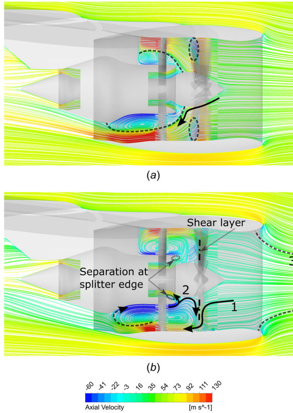
Fig. 4 Flow field evolution internal and external to the engine when the VPF transitions to reverse thrust mode [15]
