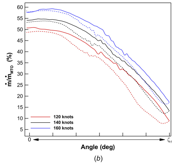
Fig. 13 Effect of aircraft landing speed on the VPF hysteresis loop: Fig. 13(a) shows the mass flowrate percentage evolution over time while Fig. 13(b) shows the VPF hysteresis loops. The forward-to-reverse thrust operations are depicted by solid lines while dashed lines represent the reverse-to-forward thrust operations.
