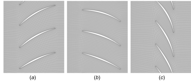
Fig. 3 Grid evolution showing the mesh deformation depicted at three stagger angles during VPF transition [15]: (a) initial forward flow position, (b) intermediate position, and (c) fully reverse thrust mode position
