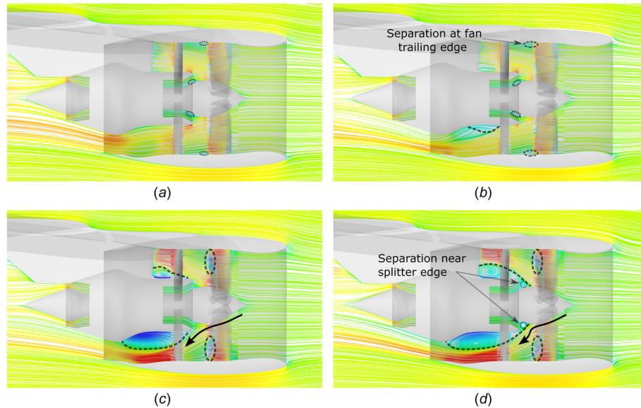
Fig. 6 Flow field evolution using axial velocity colored flow streamlines for two timestamp fan stagger angles highlighting the slower dissipation of reverse flow in the reverse-to-forward thrust operation: (a) forward-to-reverse thrust: 29 deg, (b) reverse-to-forward thrust: 29 deg, (c) forward-to-reverse thrust: 46 deg, and (d) reverse-to-forward thrust: 46 deg
