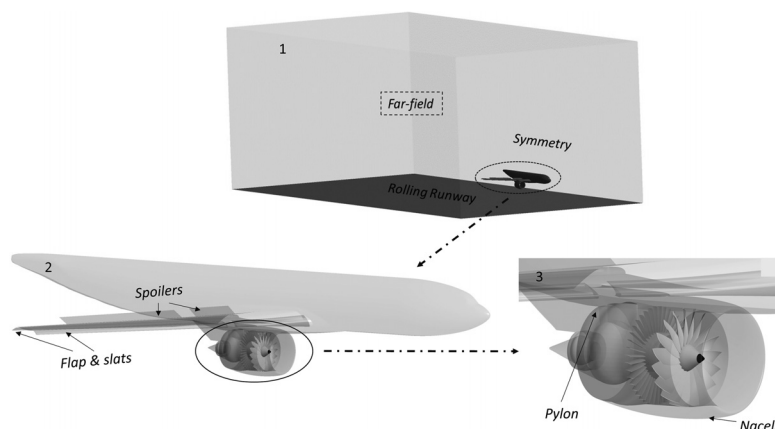
Fig. 1 Computational domain showing the integrated airframe-engine-VPF model, including the engine components [11]
