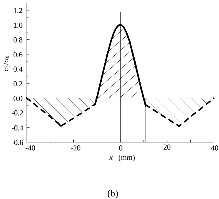
Fig. 8 Artificially balanced residual stresses: (a) with concentrated stress (case 3); (b) with distributed stress (case 4).
