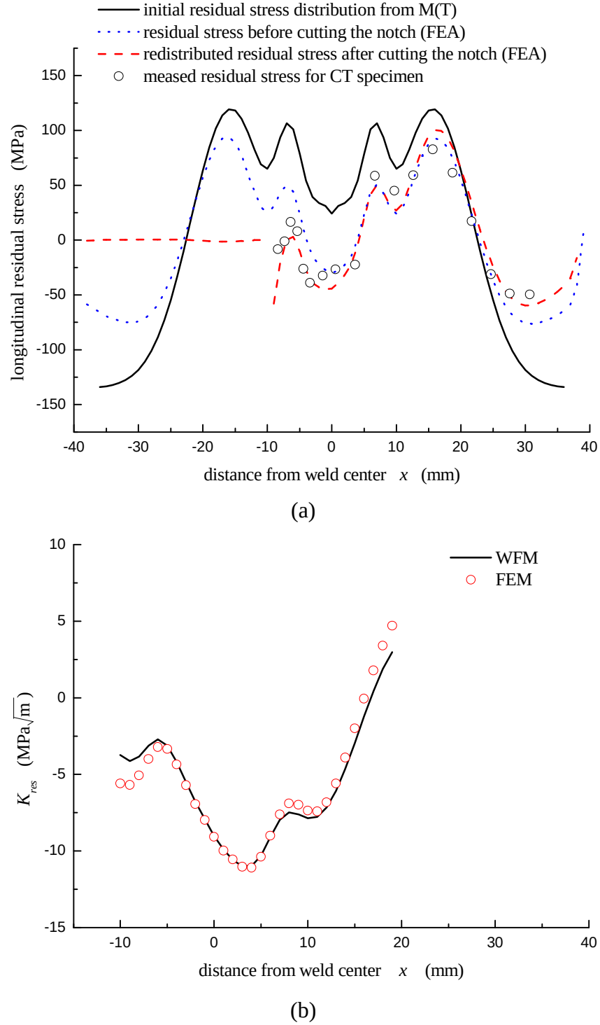
Fig. 13 (a) Residual stress redistribution in the C(T); (b) calculated K_{res} for the VPPA 2024 C(T) specimen
