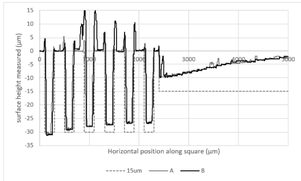
Figure 6: Form profile of Ti-30Nb square 3: DOC 15 \mu\text{m} , overlap 1, feed 250 mm/min, ss20000 rpm
