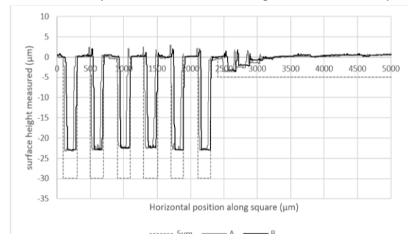
Figure 5: Form profile of Ti-30Nb square 1: DOC 5 \mu m, overlap 1.99, feed 50 mm/min, ss20000 rpm). Line A is from the left of the square, line B is from the right and the dashed line represents the targeted profile.
