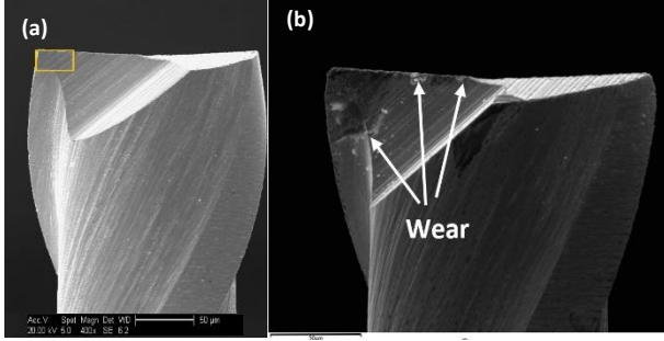
Figure 9: (a) Cutting tool before machining (b) cutting tool after machining
