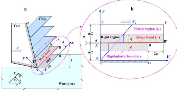
Figure 11: (a) Serrated chip flow model (b) shear band evolution model Reprinted with permission from [9], Copyright 2010 Springer
