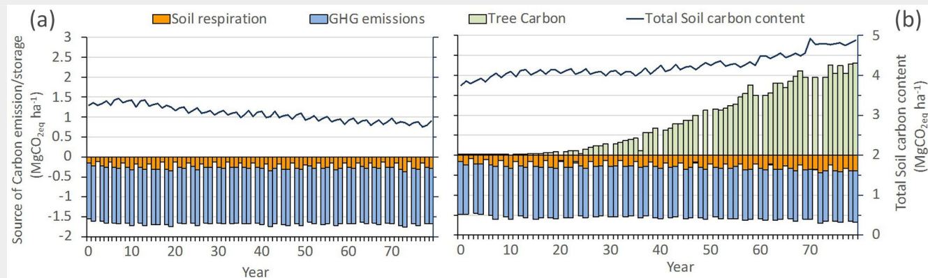
Fig. 3 - Carbon sources of emissions and storage (in Mg \text{CO}_{2\text{eq}} ha -1 ) for monoculture (a) and agroforestry (b) management systems for wheat production including emissions from soil biota respiration (soil respiration), from field operations and fertiliser, seed and pesticide production (GHG emissions) and carbon sequestered by tree (tree carbon) and stored in soil (total soil carbon content).
