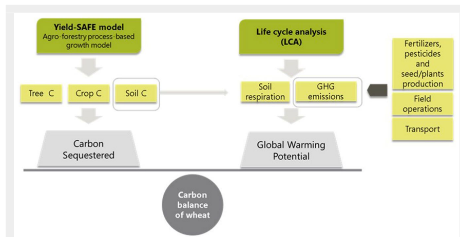
Fig. 1 - Methodology used to estimate the carbon balance of a functional unit (Mg of \text{CO}_{2\text{eq}} Mg of wheat grain -1 ) by comparing the estimation of the Yield-SAFE model of the carbon sequestered by the tree, crop and soil components and the greenhouse gas emissions derived from fertilizers, pesticides and seed/plants production, field operations, transport and soil respiration.
