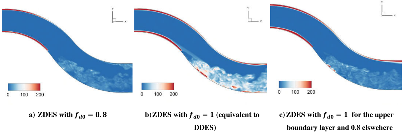
Figure 6 Instantaneous distribution of v_t/v at the symmetry plane for different f_{d0} configuration for the baseline
