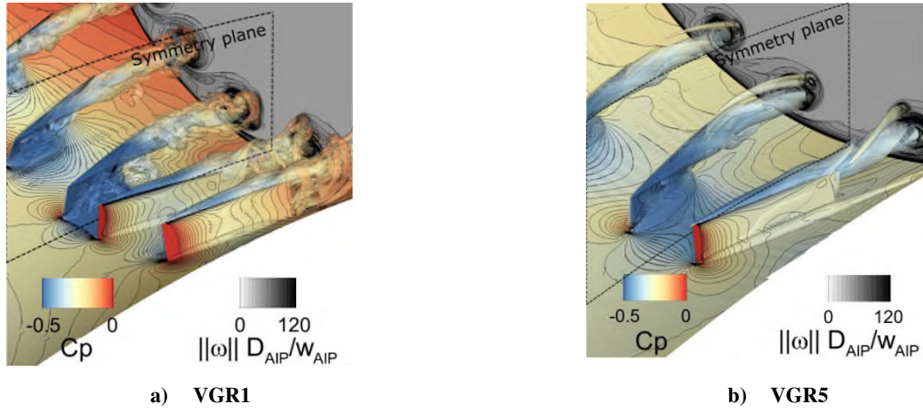
Figure 9 Visualisation of the vortex formation by Q-criteria in the VG regions. Flow direction is from left to right.
