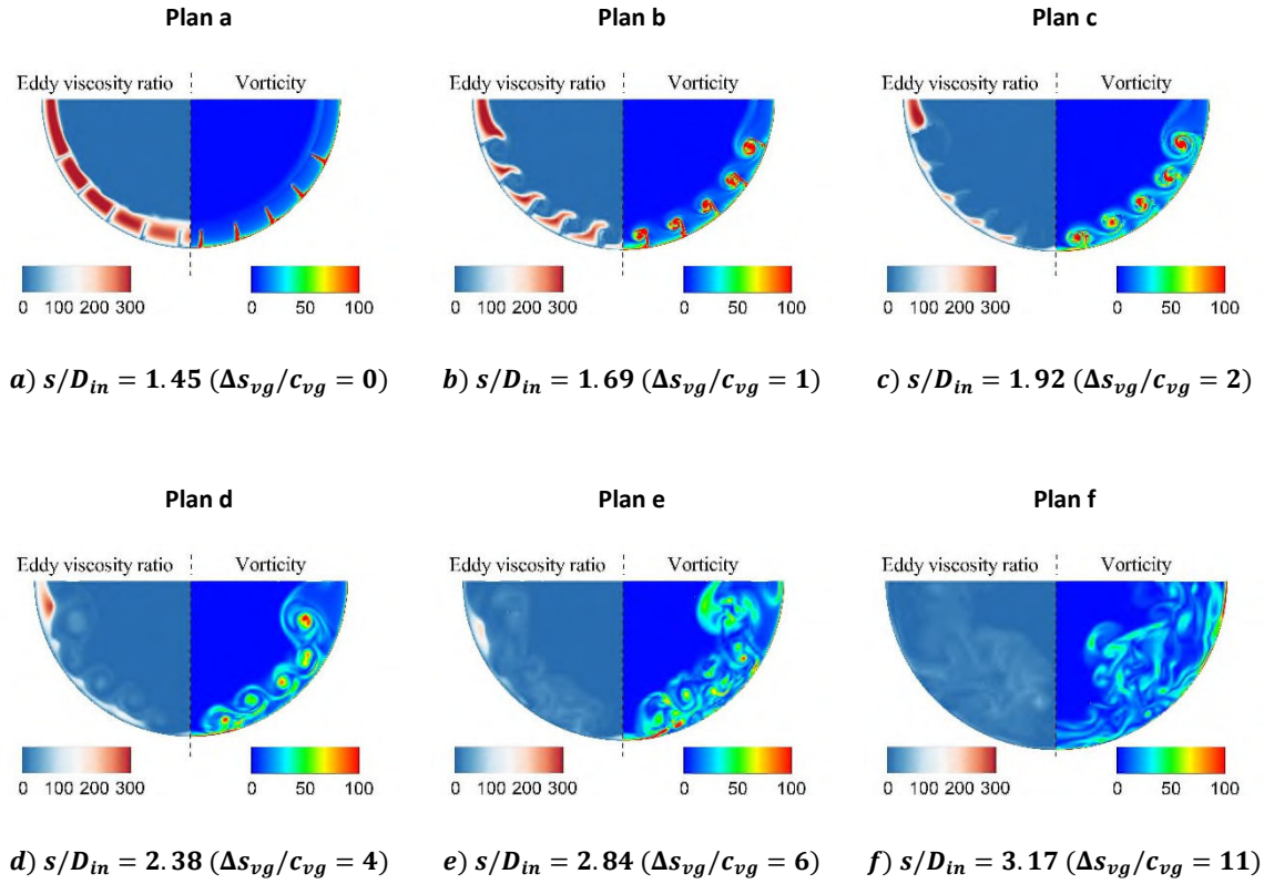
Figure 10 Instantaneous flowfield for v_t/v and |\omega|D_{in}/\langle \bar{w}_{AIP} \rangle at different cross section along the centreline s/D_{in} for the configuration VGR1. See Figure 8b for plan location a-g.
