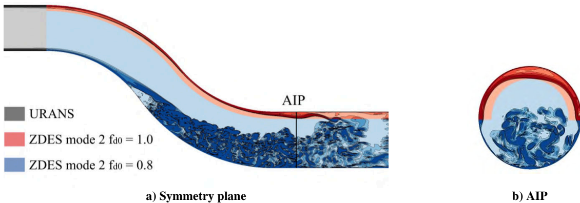
Figure 7 Instantaneous distribution of the vorticity magnitude shaded with the zonal allocation of the ZDES parameters for the baseline configuration
