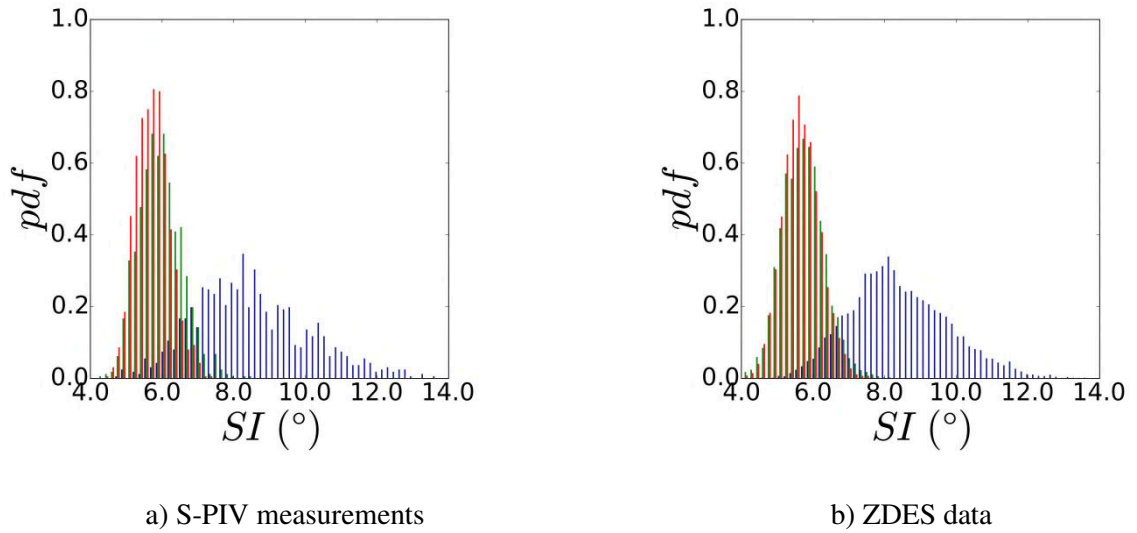
Figure 19 Normalised PDF of the Swirl intensity (SI) for the baseline (blue), VGR1 (green) and VGR5 (red) and from S-PIV and ZDES data
