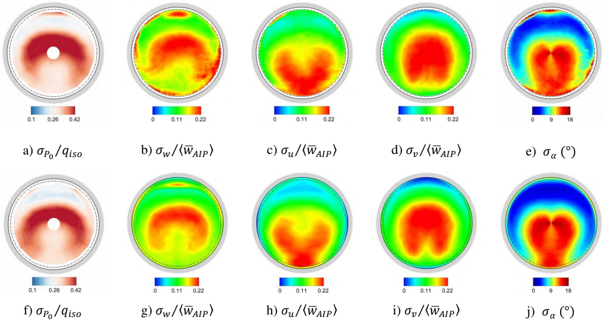
Figure 15 Flow standard deviation comparison with the experiment (top) and the ZDES (bottom). The unsteady total pressure (a) was measured with high frequency response Pitot probes, the velocity and swirl distribution are based on S-PIV data (b-e)
