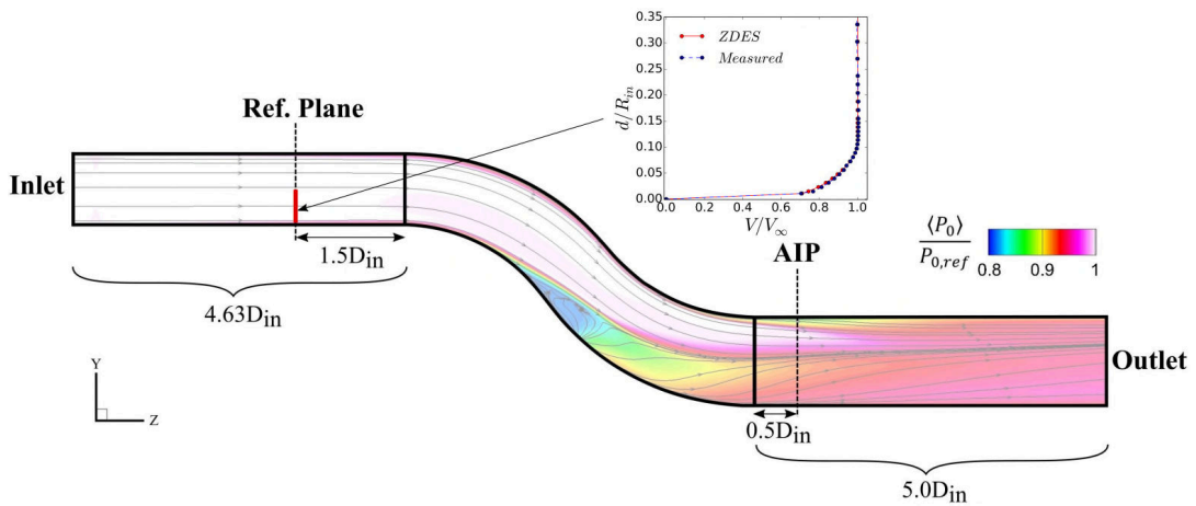
Figure 3 Illustration of the CFD domain with the baseline configuration time-averaged flow solution at the symmetry plane and boundary layer at the reference plane
