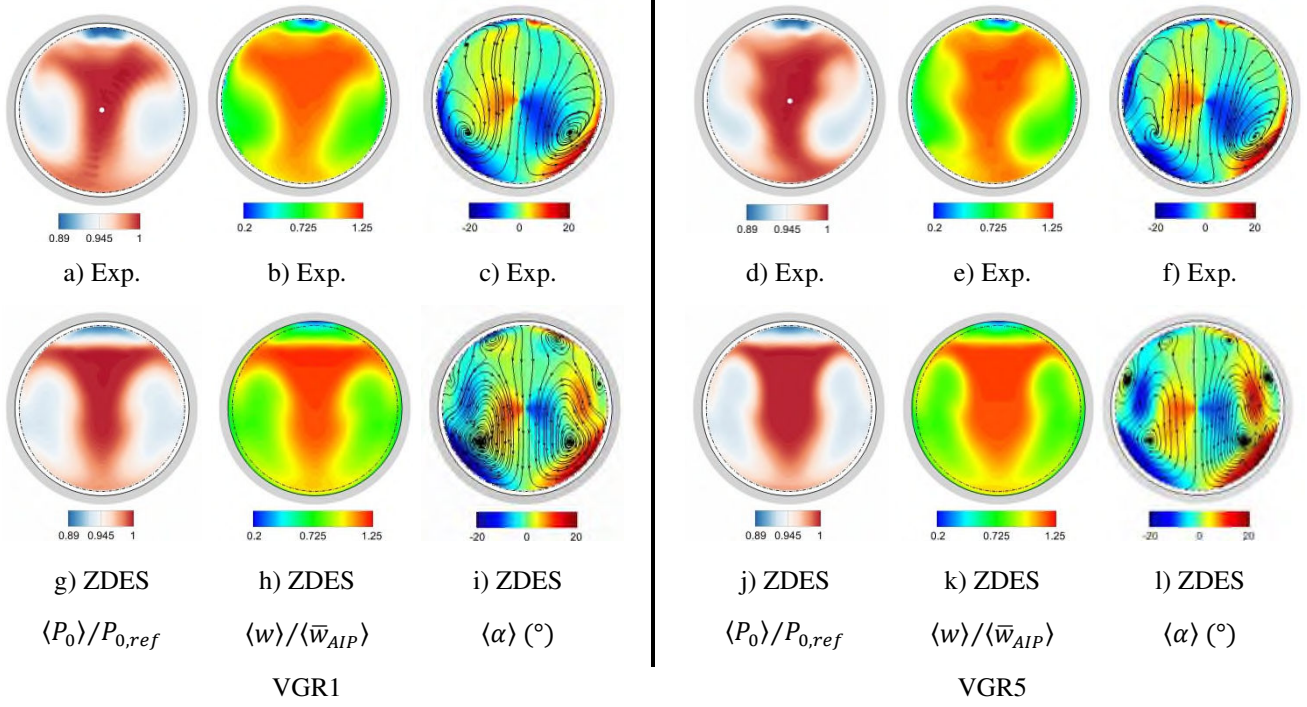
Figure 16 Comparison between the experimental (top) and ZDES time averaged flowfield with the flow control devices. The measurements are performed with steady total pressure rakes (a, d) and the S-PIV system
