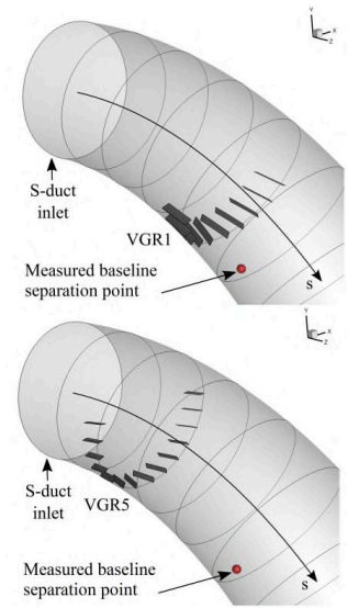
Figure 2 Illustration of the vortex generator configurations
