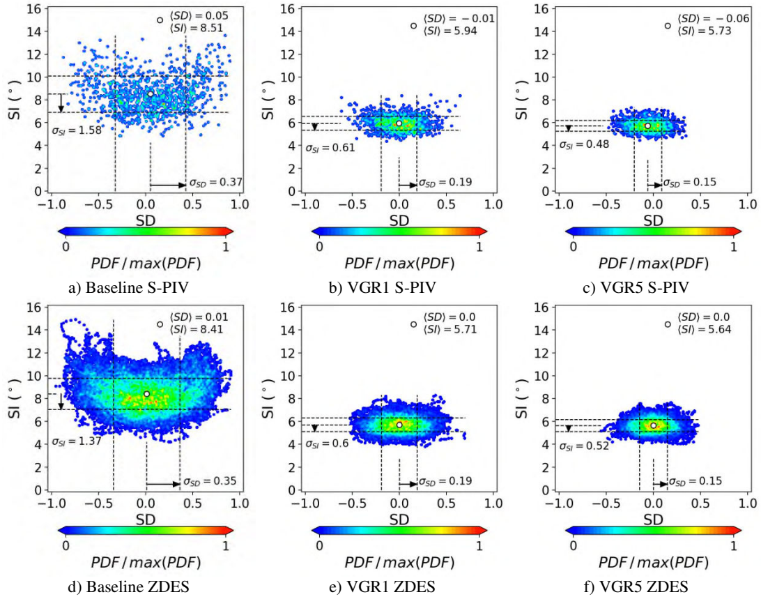
Figure 20 Comparison of the baseline and the VG configuration of the SD – SI joint probability cloud maps
