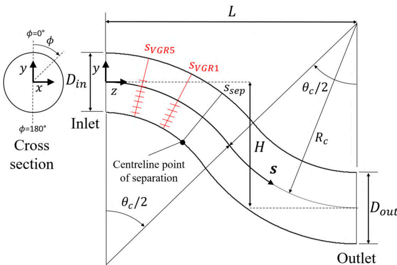
Figure 1 S-duct geometry definition
