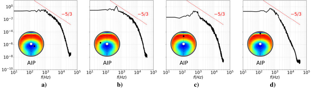
Figure 4 Power Spectral Density for the streamwise velocity at the AIP for the baseline configuration
