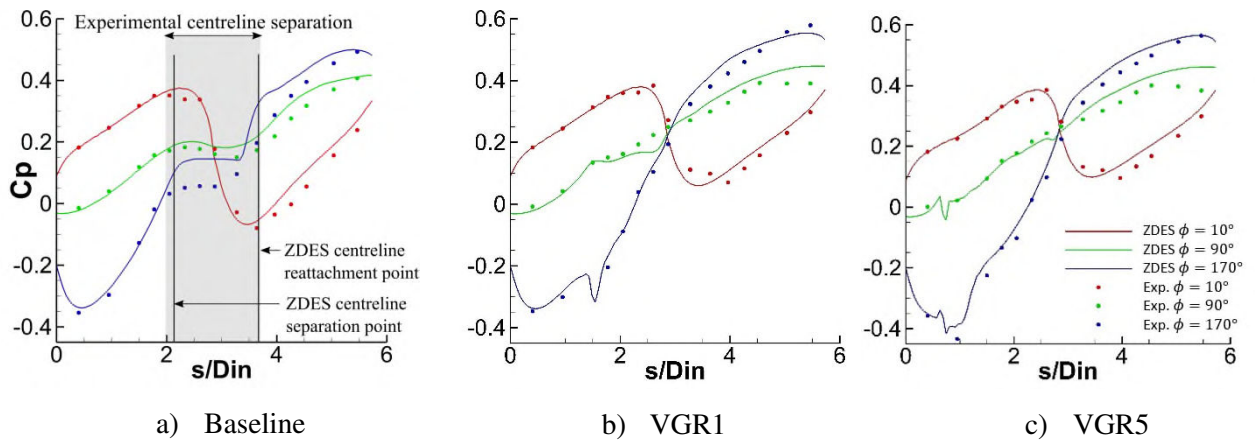
Figure 11 Comparison between the ZDES and experimental time-averaged wall static pressure coefficient within the S-duct
