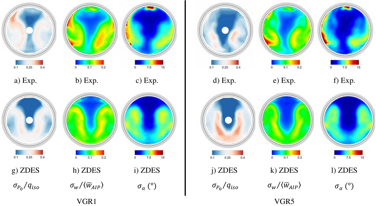
Figure 17 Comparison between the experimental (top) and ZDES fluctuating flowfield with the flow control devices. The measurements are performed with unsteady total pressure rakes (a,d) and the S-PIV system
