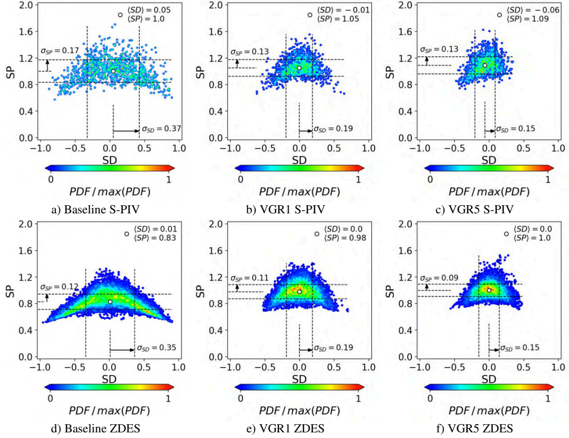
Figure 21 Comparison of the baseline and the VG configuration of the SD–SP joint probability cloud maps
