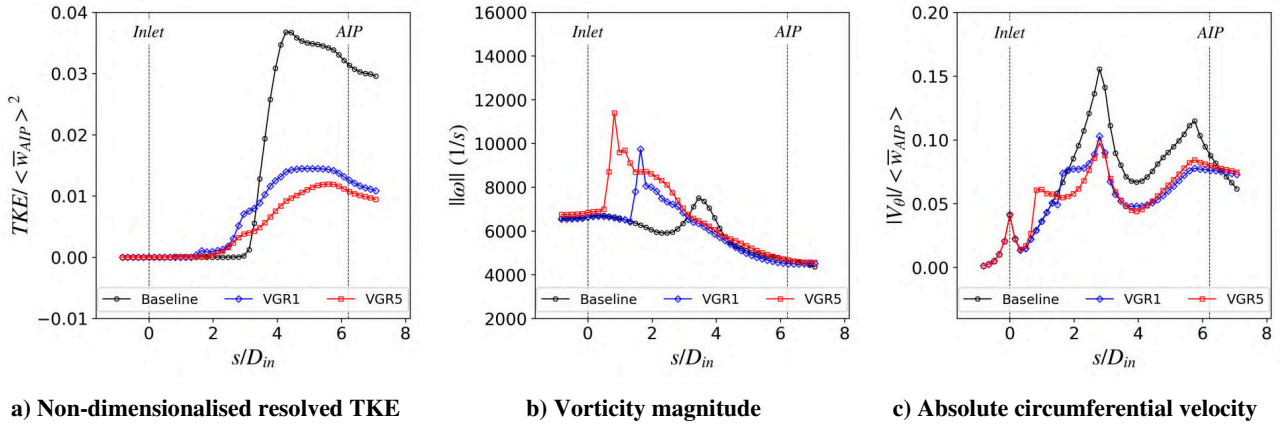
Figure 13 Streamwise distribution of the cross-sectional area-weighted average flowfield along the S-duct
