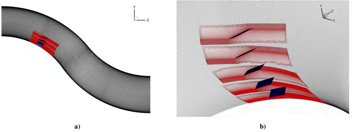
Figure 5 Representation of the Chimera mesh for VGR1
