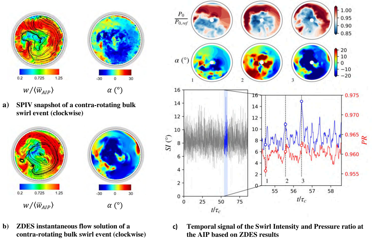
Figure 18 Illustration of the ZDES SI signal and extreme bulk swirl event at the AIP for the baseline configuration
