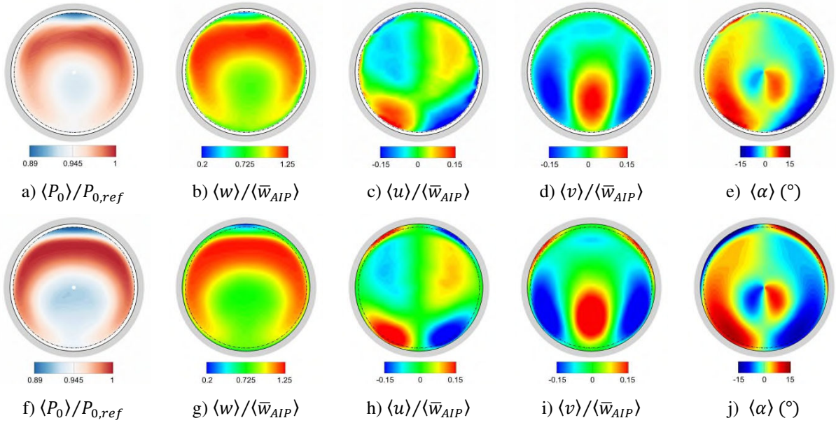
Figure 14 Flow time averaged comparison with the experiment (top) and the ZDES (bottom). The experimental total pressure (a) is based on steady measurements, the velocity and swirl distribution are based on S-PIV data (b-e)
