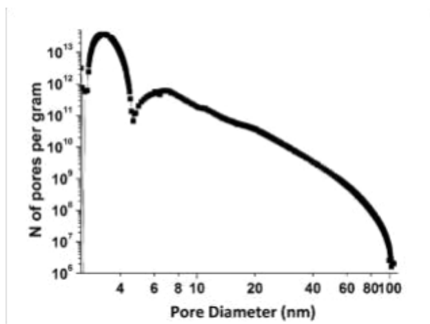
Fig.6 Pore size distribution measured by BET.
