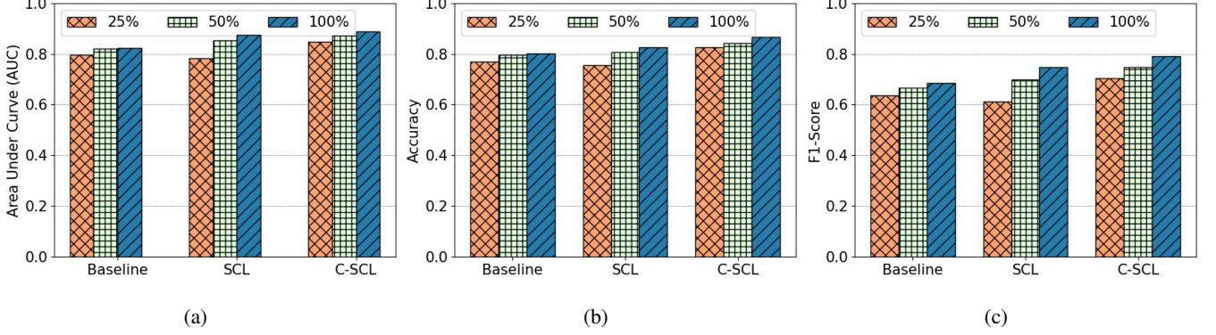
Fig. 8: Comparison of the different approaches trained on different numbers of abnormal activity samples from the DAD dataset.
