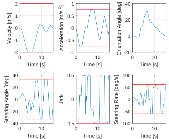
Fig. 7: Optimal trajectories for Case 4
