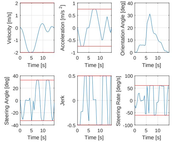
Fig. 6: Optimal trajectories for Case 3
