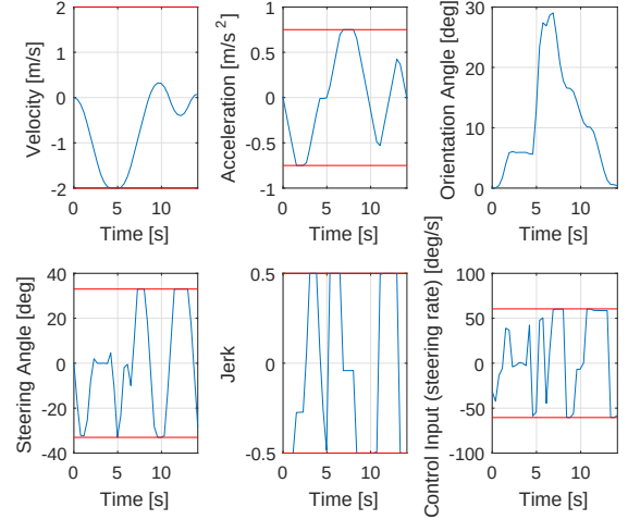
Fig. 5: Optimal trajectories for Case 1
