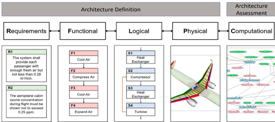
Figure 4. Requirements-Functional-Logical-Physical-Computational (RFLPC) representation of engineering systems, augmented with a computational domain (adapted from (Jimeno Altelaarrea 2021)).
