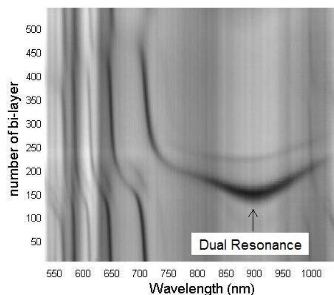
Figure 2. Grey scale plot illustrating the response of the transmission spectrum of an LPG of period 180\mu\text{m} to the deposition of a coating of calixresorcarene using the LB technique. The spectra were recorded with the LPG in the air subphase. The attenuation band originating at approximately 900 nm shows the development of the dual resonance effect.
