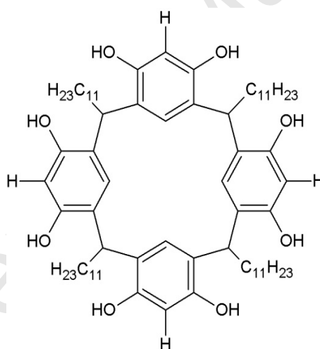
Figure 3 shows the Calixarene molecule, calix-4-resorcarene used for coating the optical fibre. The space encompassed by the larger ring forms the cavity into which the analyte molecule becomes entrapped.
