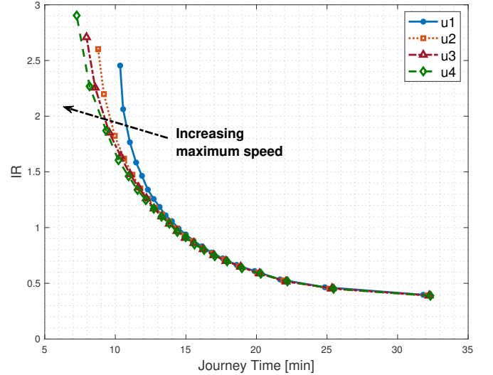
Figure 7: Pareto fronts for four driving speed showing large variation when w_m \ll w_t .
