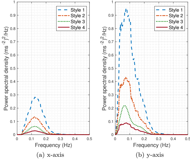
Figure 5: Frequency weighted acceleration power spectral densities in the longitudinal and the lateral axis for four driving styles.
