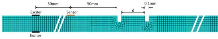
Figure 5: Two-dimensional numerical model with two notches.
