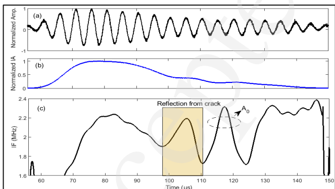
Figure 13: Instantaneous amplitude and instantaneous frequency of the damage signals: (a) original signal; (b) IA; (c) IF.
