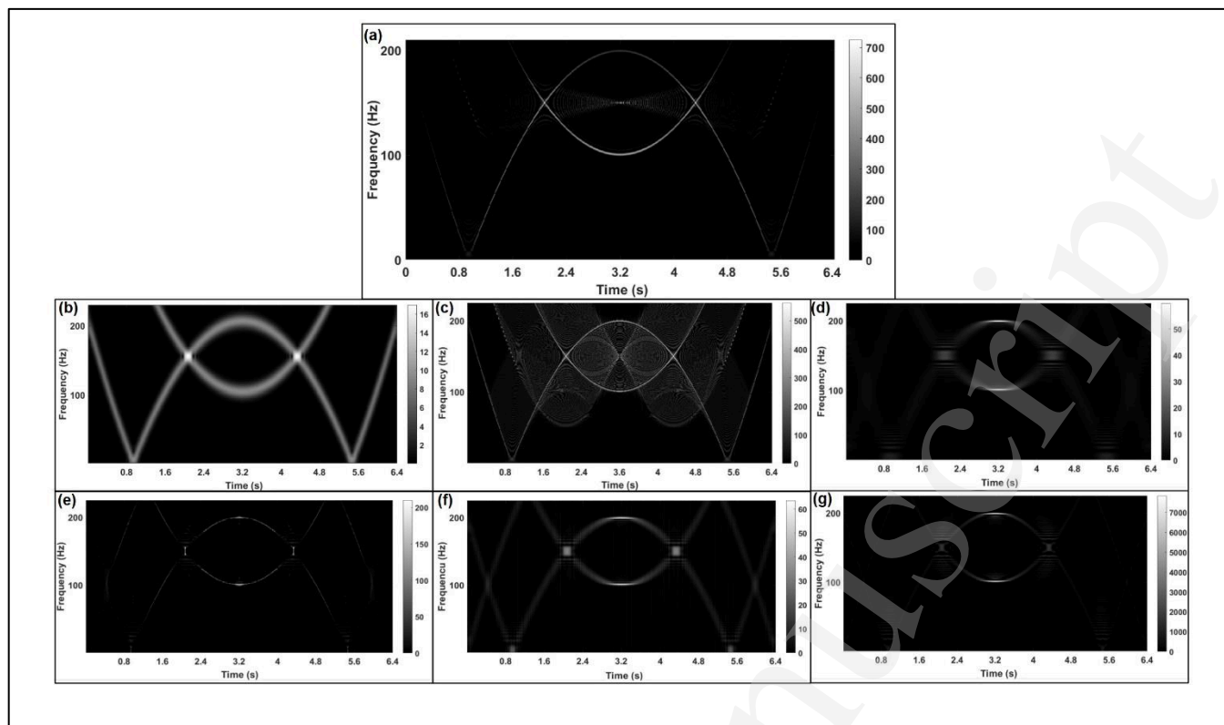
Figure 3: Time-frequency domain energy distribution: (a) proposed ME-WVD; (b) PCT; (c) WVD; (d) SPWVD (Kaiser Window, g = N/10 , h = N/4 ); (e) RSPWVD; (f) CWT ( \delta = 0.25 ) and (g) CSD.
