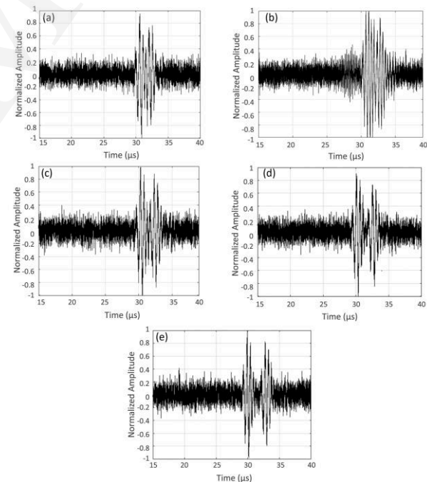
Figure 6: Reflected simulated signals from the two notches separated by: (a) 3.5mm; (b) 4mm; (c) 5mm; (d) 6mm; (e) 7mm. The signal-to-noise ratio (SNR) of all signal = 5 dB.
