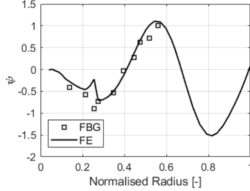
Fig. 9. FBG strain mode shape \psi for 4 th flap mode compared with FE beam models [45].
