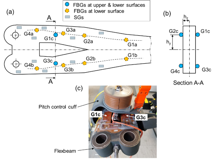
Fig. 1. (a) Diagram showing positions of the SGs and the fibre sensors deployed on the lower surface of the flexbeam, with FBGs G1a to G4a on the leading edge and G1b to G4b on the trailing edge, (b) showing fibre sensors deployed on the upper and lower surfaces of the flexbeam with FBGs G1c to G4c, (c) image of the sensor positions G1c and G3c.
