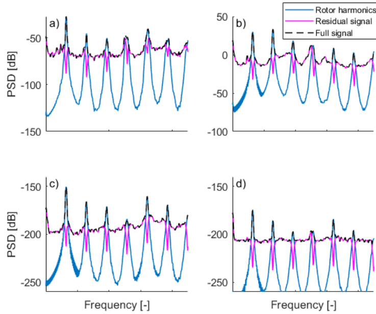
Fig. 14. Comparison of full signal, residual signal and rotor excitation for BladeSense rotor track and balance data: a) FBG sensor FBG1, b) FSI sensor S1, c) DFOSS sensor vertical, d) DFOSS sensor horizontal.
