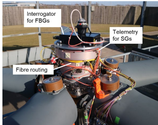
Fig. 3. Whirl-tower test: Integration of FBG strain sensors and electrical SG with their dedicated data transfer devices on a H145 (BK117 D-3) rotor blade and rotor head.
