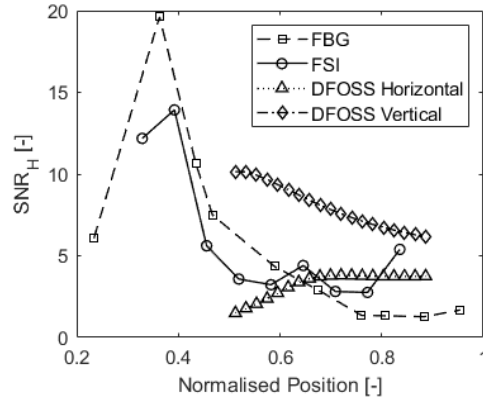
Fig. 13. Comparison of signal-to-noise ratio SNR_H of FBG, DFOSS and FSI sensors for BladeSense rotor track and balance data.
