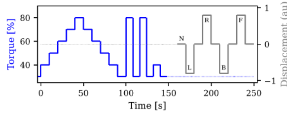
Fig. 6. Planned pilot input pattern to the collective and cyclic controls; stepped collective (0–100 s), collective doublet (100–150s), doublet cyclic lateral (160–200) and doublet cyclic longitudinal (200–250 s), N—neutral, L—left, R—right, B—backward, F—forward [16].
