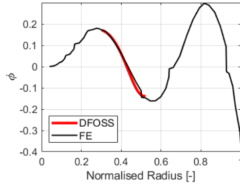
Fig. 10. DFOSS displacement mode shape \phi for 4 th flap mode compared with FE beam models [45].
