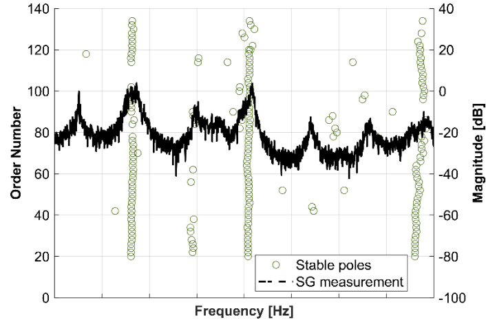
Fig. 7. Stabilisation diagram for sensors in flap direction computed with the following parameters: \Delta f = 1\% , \Delta \zeta = 5\% , \Delta MAC = 0.98 for one realisation of SG measurements from the WTT track and balance run.
