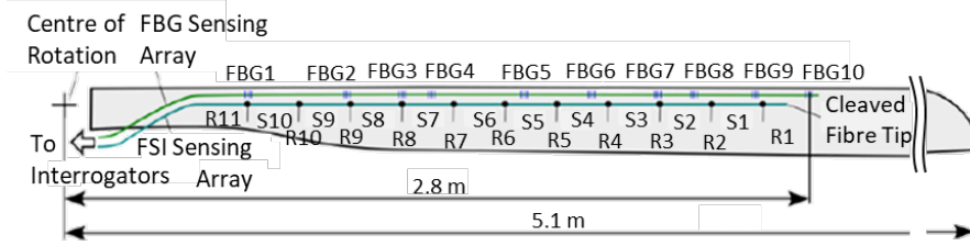
Fig. 2. Diagram showing positions of the fibre sensors deployed on the lower surface of the rotor blade, with FBGs G1 to G10 and FSI sensing segments S1 to S10 shown. The black dots in the FSI sensor array represent the locations of the FSI reflectors, R1 to R11.
