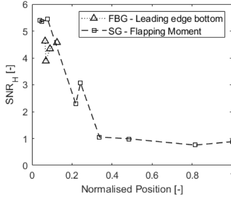
Fig. 11. Comparison of signal-to-noise ratio SNR_H for H145 WTT rotor track and balance data: triangles: FBG sensors, G1a - G4a, on bottom leading edge position; squares: SG sensors, flapping moment.
