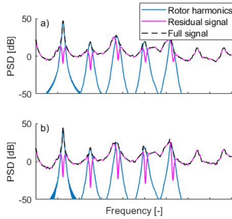
Fig. 12. Comparison of full signal, residual signal and rotor excitation for H145 WTT rotor track and balance data: a) FBG sensor G2a, b) SG sensor MB320.
