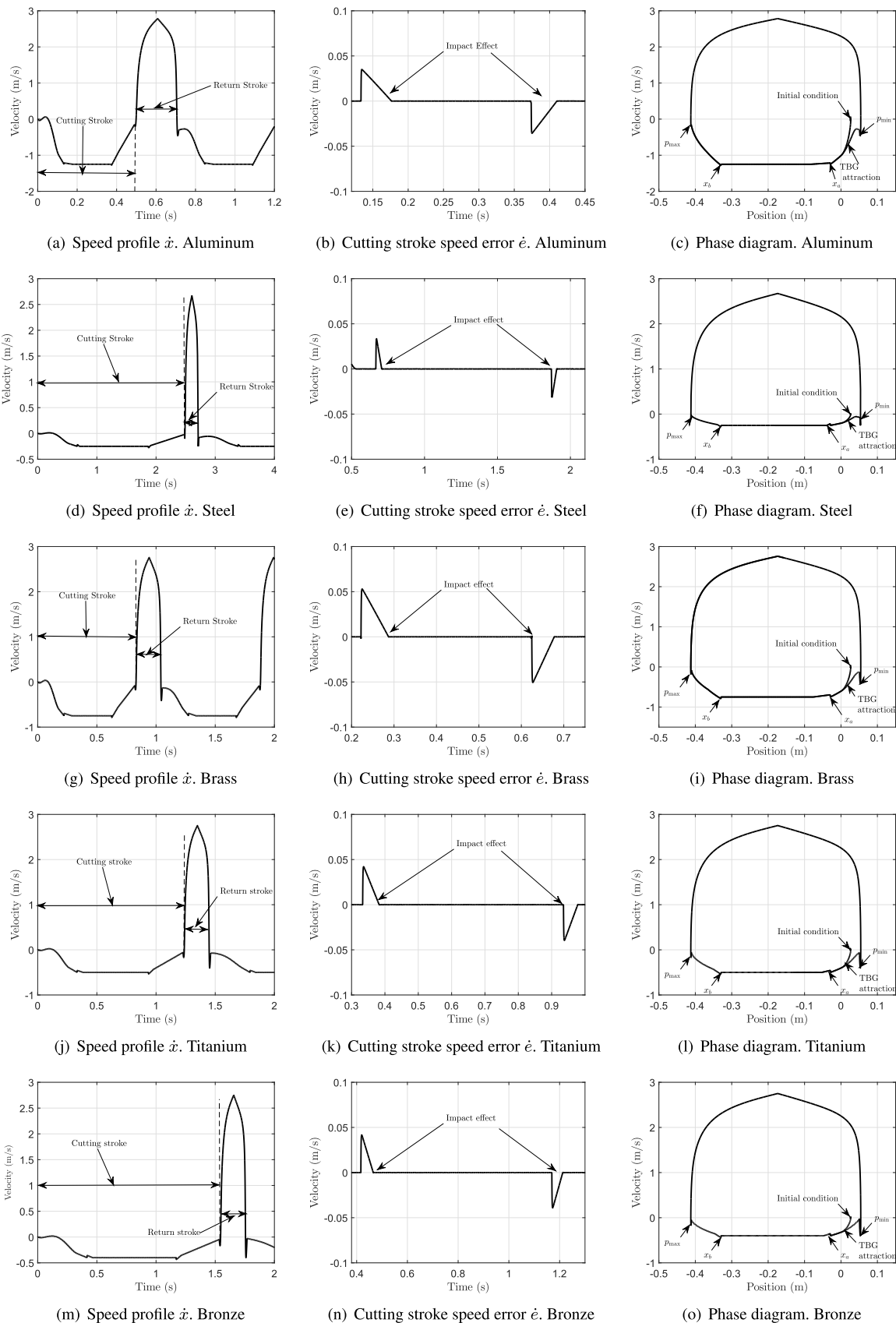
FIGURE 10. Speed profile \dot{x} , Cutting stroke speed error \dot{e} , Phase diagram of each material under the parameters of Table 1.
