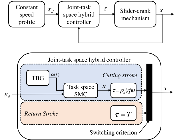
FIGURE 1. Closed-loop system diagram of the proposed approach.
