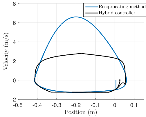
(b) Phase diagram comparisons
