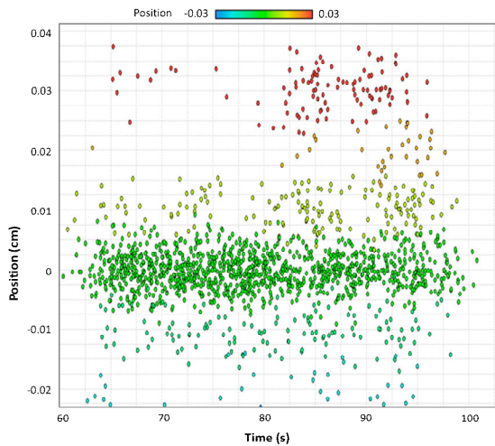
Figure 6: Position of mobile robot with the factor for the rotational velocity at 0.15m/s
