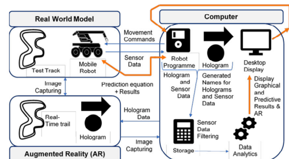
Figure 2: Mobile Robot DT Architecture
