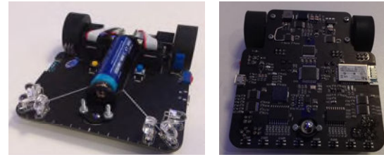
Figure 3: (a) Front side of mobile robot, (b) Back side of the developed mobile robot
