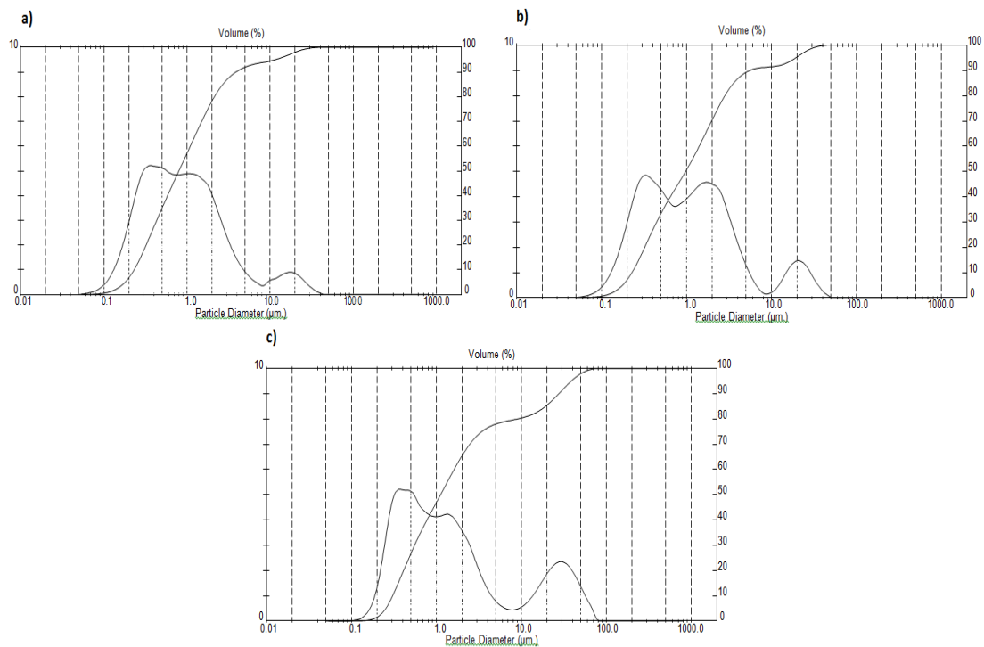
Figure 2: Particle size distributions of carbonation precipitates as a function of temperature (18.5 g \text{Ca(OH)}_2 , MCR = 3, reaction volume = 250 ml): a) T = 30 °C, b) T = 50 °C, and c) T = 70 °C.
