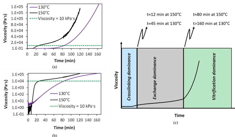
Fig. 7. Rheological behaviour of DHPDS-a during cure. (a) Viscosity versus time. (b) Viscosity in log scale versus time. (c) Regimes of dominance of crosslinking, bond exchange, and vitrification.
