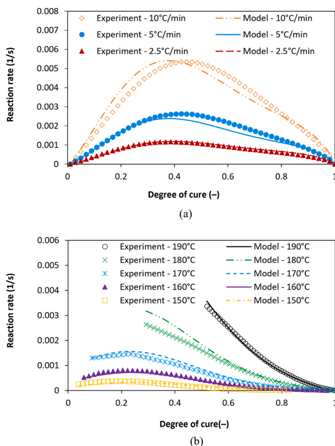
Fig. 5. Cure kinetics modelling of DHPDS-a: Comparison of model and experiment reaction rate in dynamic (a) and isothermal (b) conditions.
