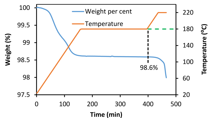
Fig. 1. TGA thermogram of DHPDS-a benzoxazine monomer.
