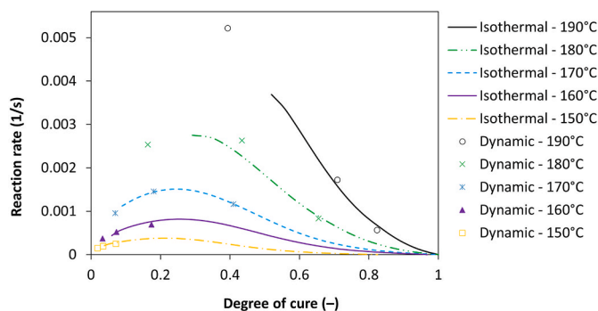
Fig. 4. Superposition of dynamic and isothermal reaction rate versus degree of cure data for DHPDS-a vitrimer.
