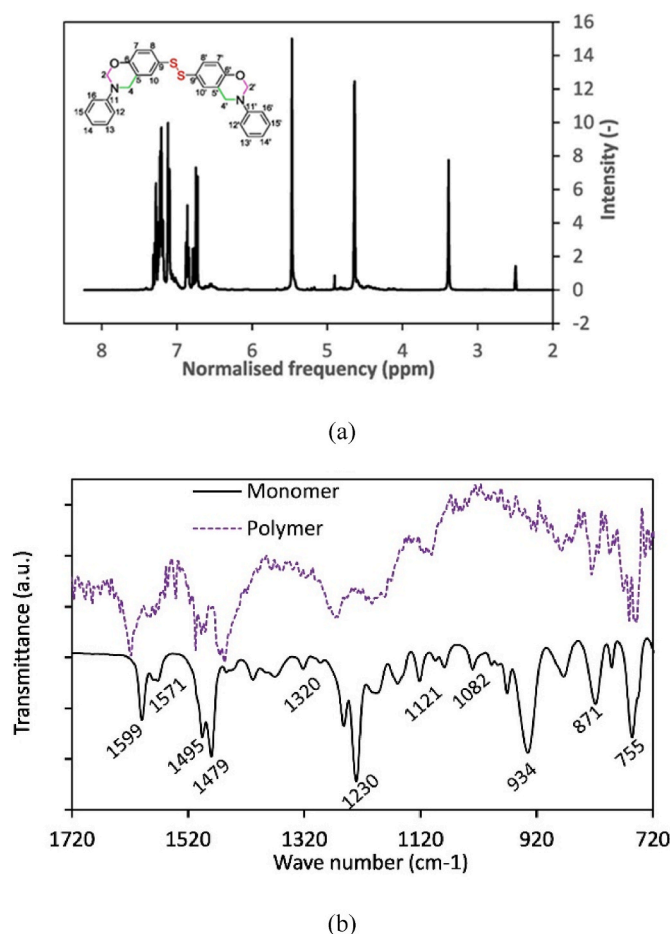
Fig. 3. ^1\text{H} NMR and FTIR spectra of DHPDS-a benzoxazine vitrimer. Reproduced from Ref. [27]. Copyright 2025, Elsevier.
