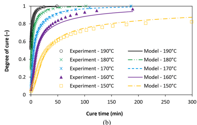
Fig. 6. Cure kinetics modelling of DHPDS-a: Comparison of model and experiment degree of cure evolution in dynamic (a) and isothermal (b) conditions.
