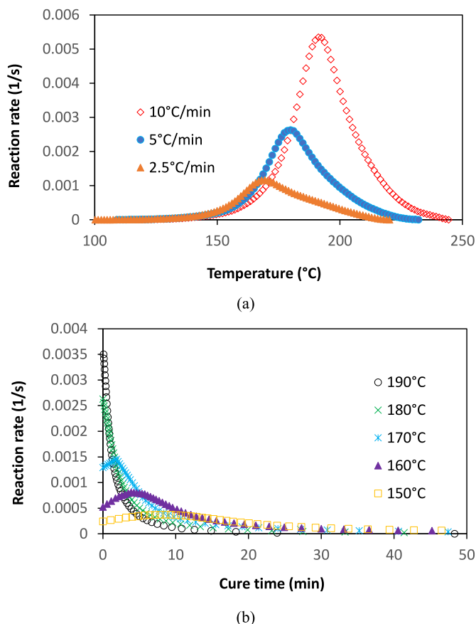
Fig. 2. Experimental cure kinetics of DHPDS-a system: (a) reaction rate versus temperature in dynamic DSC experiments; (b) reaction rate versus cure time in isothermal DSC experiments.
