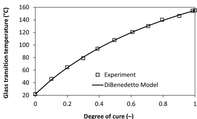
Fig. 8. Dependence of glass transition temperature of DHPDS-a vitrimer on degree of cure.
