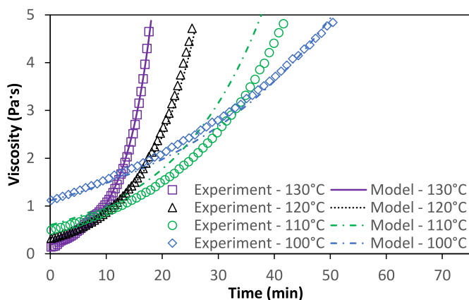
Fig. 9. Viscosity evolution of DHPDS-a over time at various isothermal temperatures and comparison of model to experiment.
