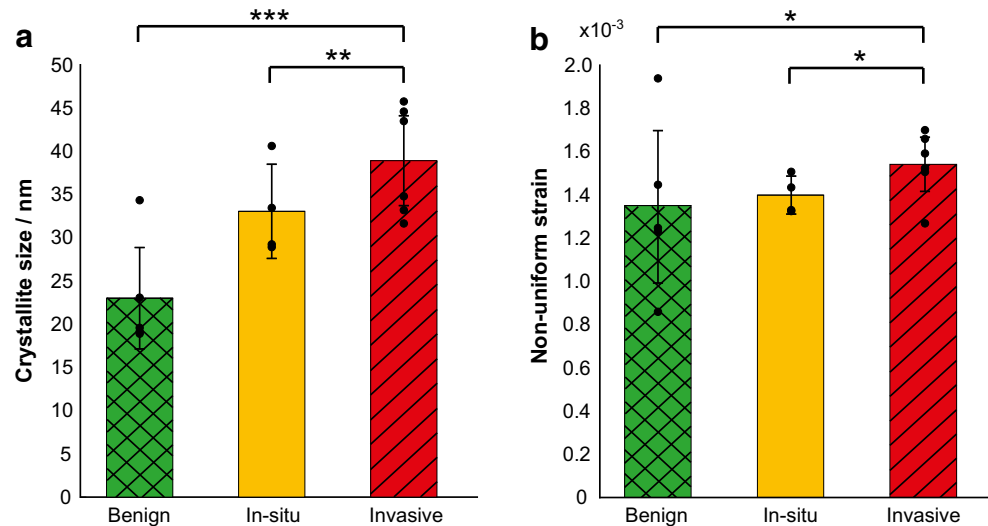
Fig. 4 Crystallite size (a) and non-uniform strain (b) measurements for benign ( n = 5 ), in-situ ( n = 4 ) and invasive ( n = 6 ) calcifications in the 001 direction. Marked points indicate the average value for each sample. Statistical analysis was carried out using Mann-Whitney U test, *P < 0.05 , **P < 0.01 , ***P < 0.001 . Error bars represent 95% confidence intervals
