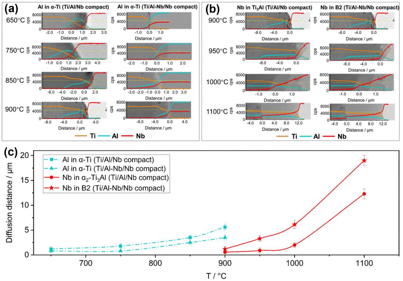
Fig. 17 EDS patterns at the interfaces of (a) Ti and Al, and (b) Nb and \text{Ti}_3\text{Al} /B2 for the Ti/Al/Nb and Ti/Al-Nb/Nb compacts quenched at 650-1100 °C. (c) Measured diffusion distance of Al in \alpha -Ti, Nb in \alpha_2 - \text{Ti}_3\text{Al} , and Nb in B2.
