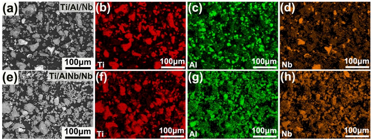
Fig. 1 (a) SEM image and (b)-(d) element mappings of the ball milled Ti/Al/Nb powders, (e) SEM image and (f)-(h) element mappings of the ball milled Ti/Al-Nb/Nb powders.
