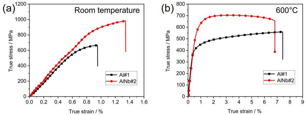
Fig. 5 True stress-strain curves of the pressurelessly sintered Ti-Al-Nb alloys at (a) room temperature and (b) 600 °C.
