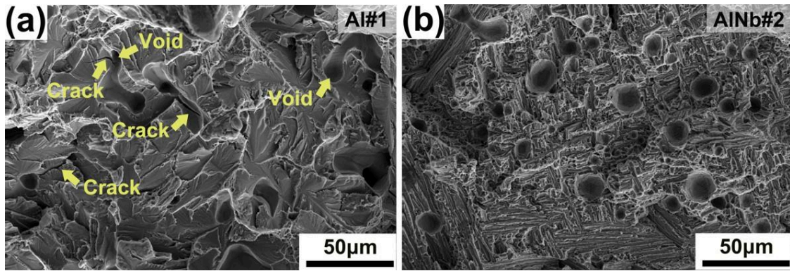
Fig. 6 Fracture morphologies of the Ti-Al-Nb alloys prepared from (a) elemental Al powder (Al#1) and (b) Al-Nb master alloy powder (AlNb#2) after room-temperature tensile tests.
