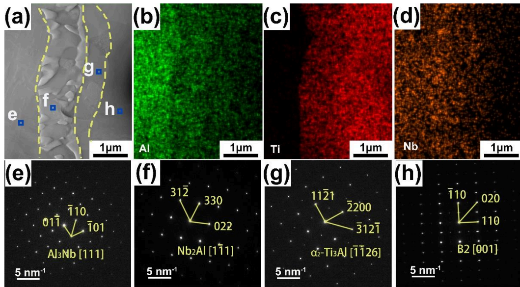
Fig. 14 (a) HADDF image, (b)-(d) element mapping of the Ti/Al/Nb compact quenched at 950\ ^\circ\text{C} , and (e)-(h) SAED patterns of the corresponding regions in (a).
