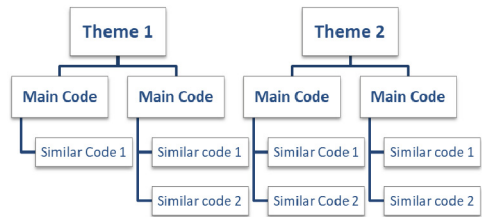
Fig. 1. Coding structure
