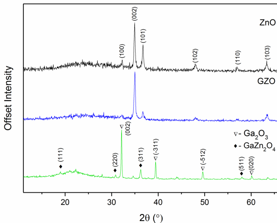
Fig 5: XRD spectra of ZnO on glass (black); GZO film deposited on glass (blue) and GZO on quartz annealed at 1000°C (green). Diamond markers in the annealed spectrum show where Bragg peaks occur characteristic of zinc gallate, triangle markers show Ga_2O_3 .
