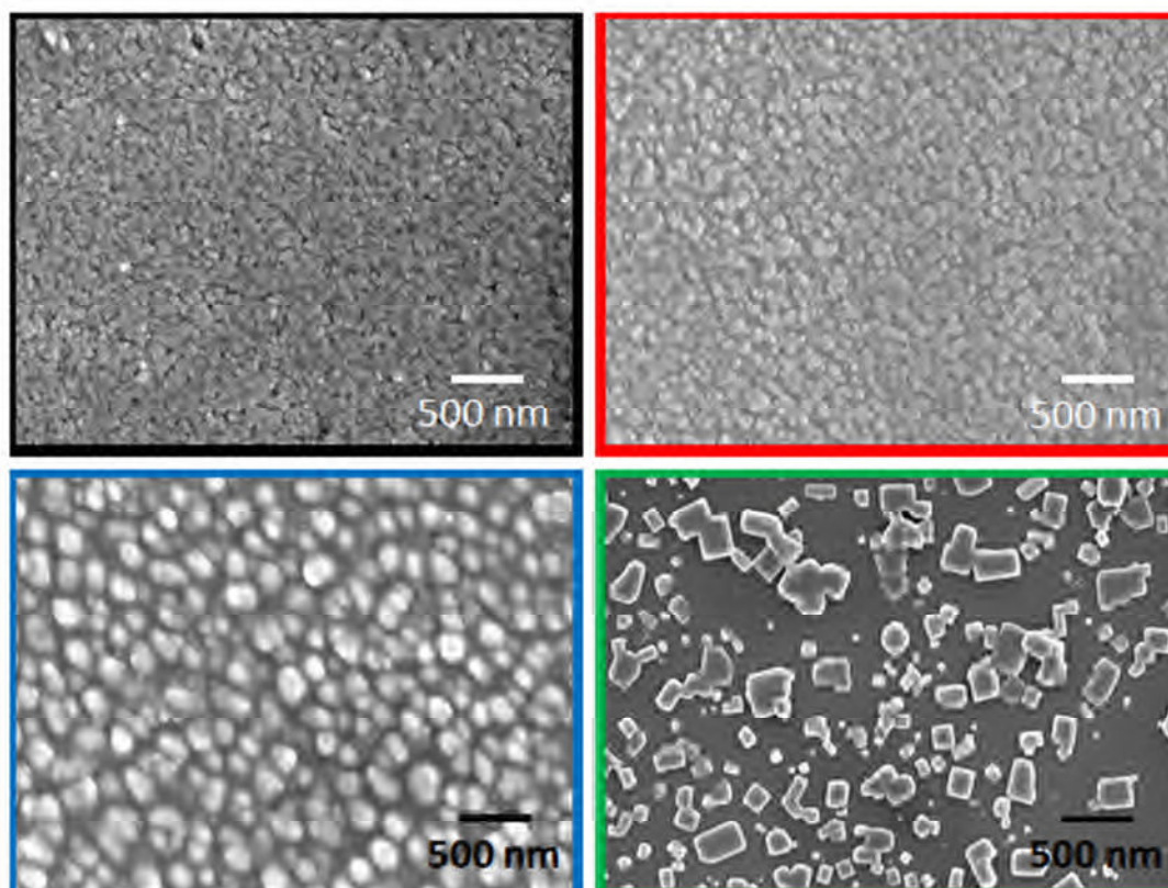
Fig. 4: SEM images of thin films grown at 400°C of: ZnO deposited from 1 (black border); b) AZO deposited from a one-pot mixture of 1 and 2 (red border); GZO deposited from a one-pot mixture of 1 and 3 (blue border); and the crystalline spinel: GaZn 2 O 4 produced from heating GZO thin films on quartz substrates at 1000°C (green border).
