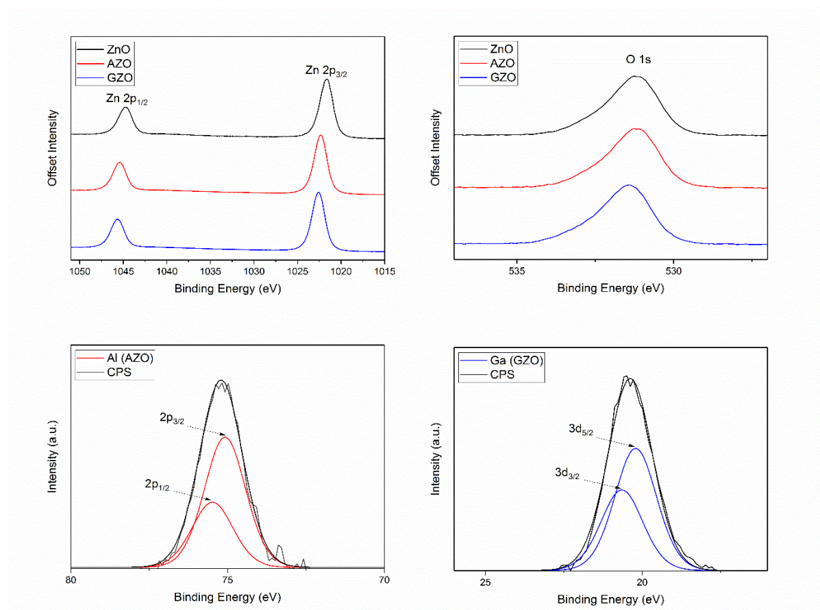
Fig. 2: XPS analysis of: Zn 2p peaks in ZnO (black), AZO (red) and GZO (blue) (top left); O 1s peaks in ZnO (black), AZO (red) and GZO (blue) (top right); Al 2p in AZO (red) (bottom left); and Ga 3d in GZO (blue) (bottom right).
