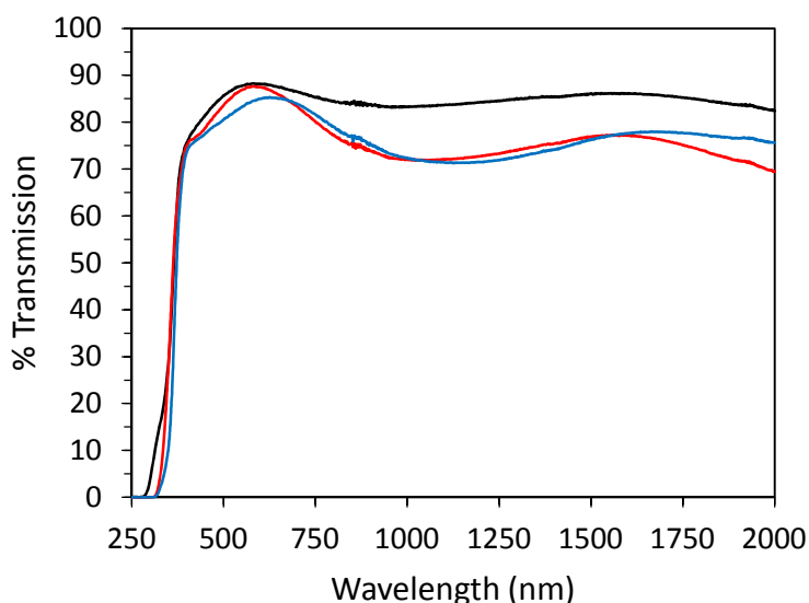
Fig. 3: UV/vis data for ZnO thin film deposited from 1 at 400°C (black); AZO film deposited from 1 and 2 at 400°C (red); GZO film deposited from 1 and 3 at 400°C (blue).
