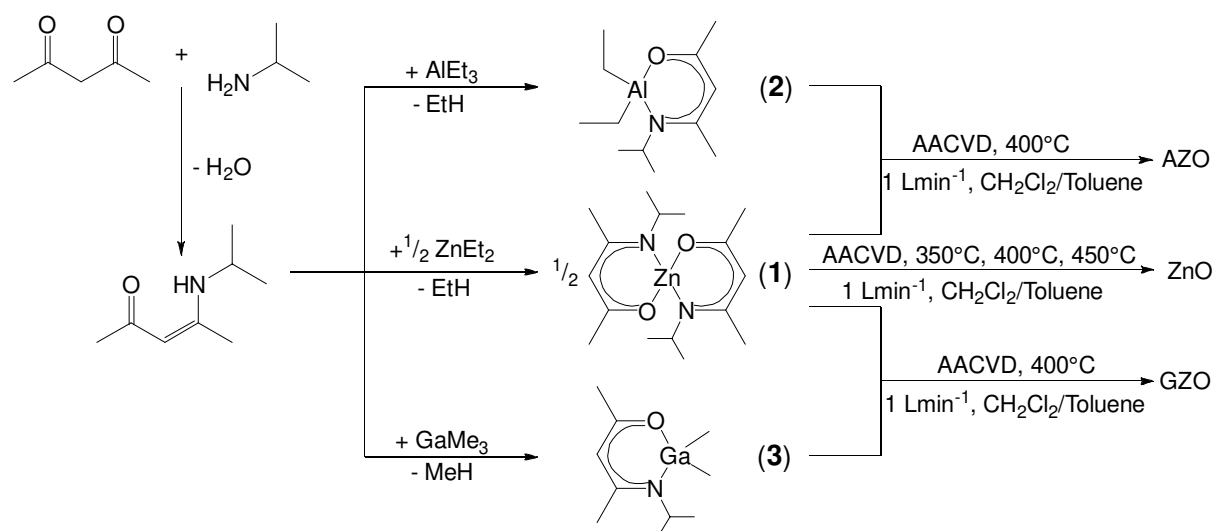
Scheme 1. Synthesis of β-ketoiminate metal complexes 1-3 and the conditions for the AACVD of thin films of ZnO, AZO and GZO.
