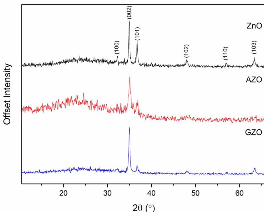
Fig. 1: XRD pattern showing: ZnO deposited by AACVD of 1 at 400°C (black); AZO deposited from 1 and 2 (red); GZO deposited from 1 and 3 (blue). Peaks verify the hexagonal wurzite structure expected.
