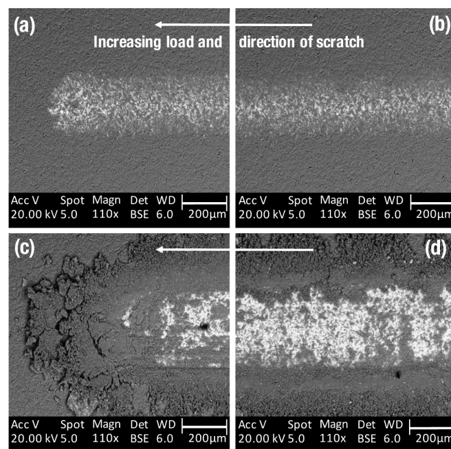
Figure 6. SEM images of a wear scar on a sample with 9% and 35% TiB 2 (images (a,b) showing the finish and middle sections of the scratch) and a sample with 35% TiB 2 (images (c,d) showing the finish and middle sections of the scratch). The arrow shows the direction of the scratch.
