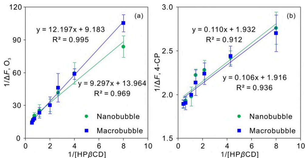
Fig. 4. Benesi-Hildebrand plots for O_3 and 4-CP in macrobubble and nanobubble aerated solutions at different HP\beta CD:O_3 molar ratios (0.5:1 to 15:1). The lines represent regression results used for binding equilibrium analyses.
