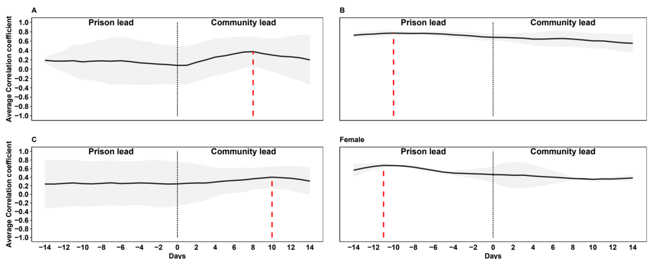
Fig. 4. Lead/lag analysis of SARS-CoV-2 concentration levels in prison and community wastewater by type of prison. (A) High-security prisons; (B) Local or training prisons; (C) Training and resettlement prisons; Female - closed women-only prison. The grey shadow represents the standard deviation. The dashed red line indicates the time when the correlation coefficient is highest.
