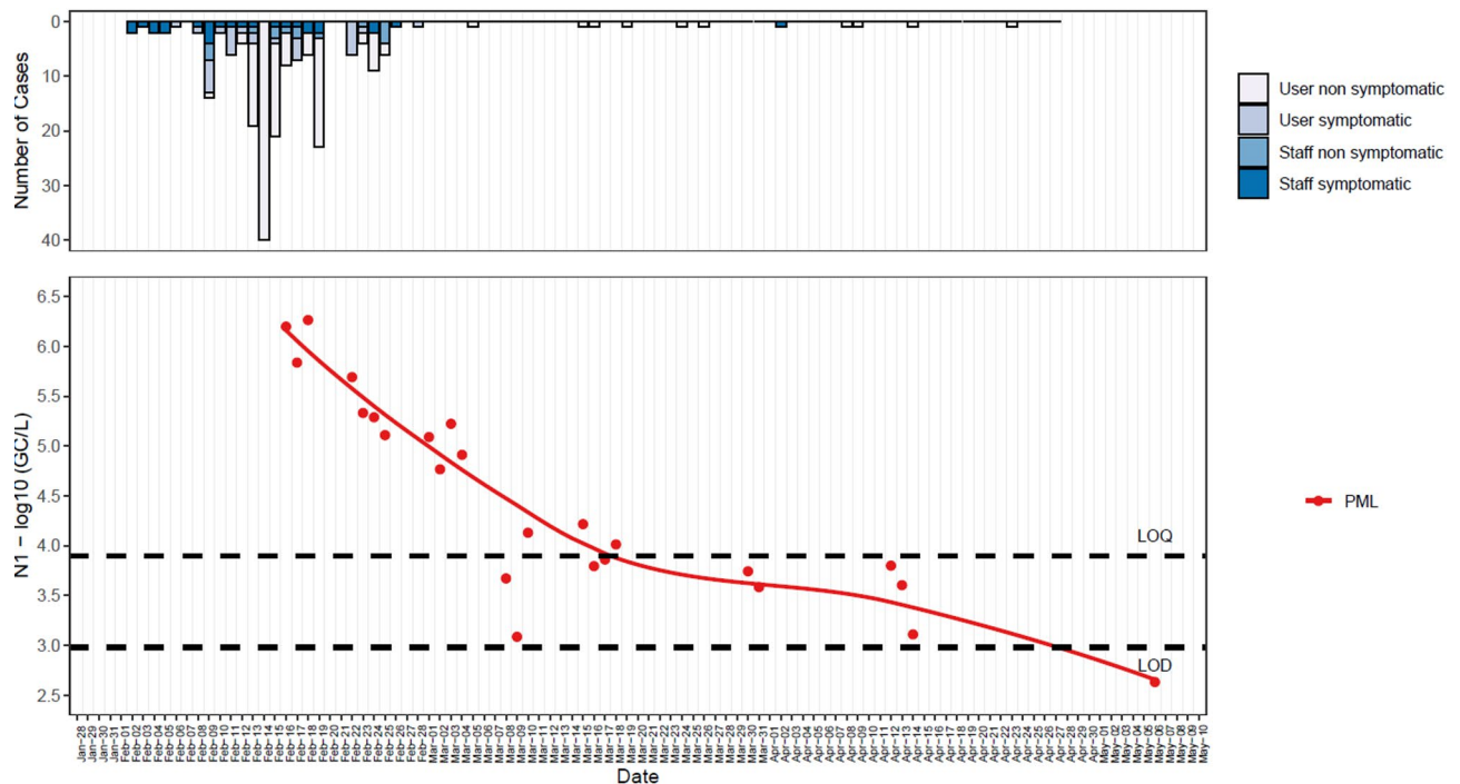
Fig. 2. Association between COVID-19 case counts and wastewater viral loads during the declining phase of the outbreak at PML. Top Panel: Daily number of new COVID-19 cases. Mass testing events on April 1 and April 8 2021. Bottom Panel: SARS-CoV-2 N1 gene segment concentrations (log10 genomic copies per litre, GC/L) in wastewater. Each point represents the log-transformed concentration from PML. The LOESS (Locally Estimated Scatterplot Smoothing) regression lines depict trends. LOQ: limit of quantification; LOD: limit of detection.
