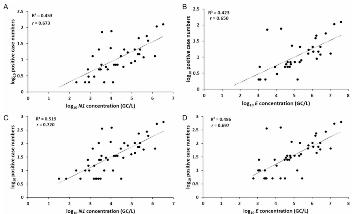
Fig. 3. Correlation between weekly clinical cases and SARS-CoV-2 wastewater concentrations. Relationship between positive COVID-19 case numbers (excluding mass testing data) and wastewater concentrations of SARS-CoV-2 N1 and E genes (GC/L). Panels A and B consider log transformed weekly case data and average weekly wastewater concentrations. Panels C and D consider corrected case numbers considering the 5-fold under-reporting ratio calculated through mass testing data. Correlation measure with Spearman's rank correlation coefficient ( r ).
