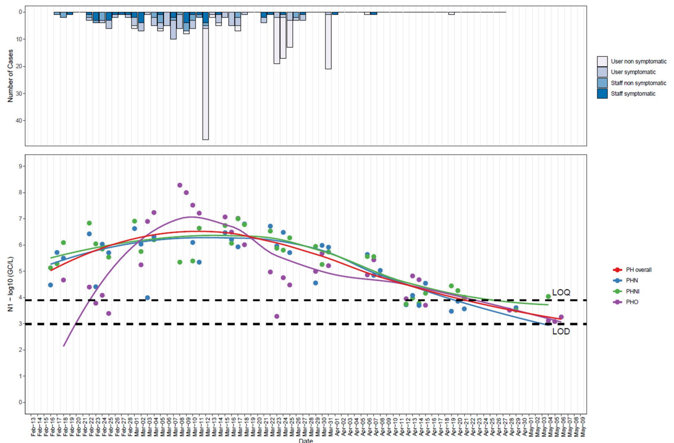
Fig. 1. Relationship between COVID-19 clinical cases and wastewater viral loads. Top Panel: Daily number of new COVID-19 cases. Targeted mass testing on March 12 and comprehensive mass testing across the entire prison on March 23, 24, 25, and 31. Bottom Panel: SARS-CoV-2 N1 gene segment concentrations (log 10 genomic copies per litre, GC/L) in wastewater. Each point represents the log-transformed concentration from two sampling sites (PHN and PHO) collected overnight and a high-frequency sampling site (PHNI) with samples collected every 5 min from 07:00–09:00. The LOESS (Locally Estimated Scatterplot Smoothing) regression lines depict trends for each site: blue for PHN, purple for PHO, and green for PHNI, with the overall trend shown in red. LOQ: limit of quantification; LOD: limit of detection.
