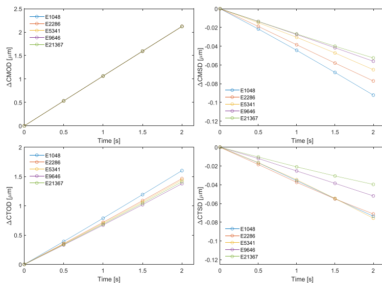
FIGURE A2 Opening (left) and sliding (right) components of the \Delta\text{CMD} and \Delta\text{CTD} under displacement control for five meshes with different refinement. The label and color correspond to the number of elements in the simulation [Colour figure can be viewed at wileyonlinelibrary.com ]
