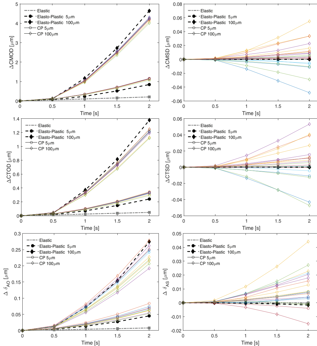
FIGURE 8 Opening (left) and sliding (right) components of the \Delta\text{CMD} , \Delta\text{CTD} , and \Delta\delta_A under force control. Colors correspond to 10 equiaxed microstructural realizations, while black corresponds to homogeneous isotropic plastic model [Colour figure can be viewed at wileyonlinelibrary.com ]
