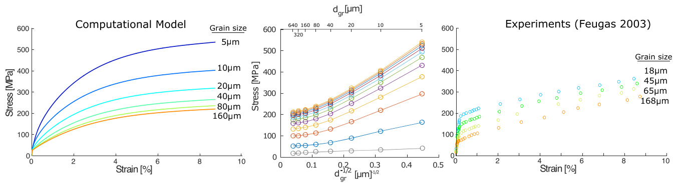
FIGURE 3 Engineering stress-strain curves for various grain sizes from crystal plasticity models (left and center) and experiments 64 (right) [Colour figure can be viewed at wileyonlinelibrary.com ]
