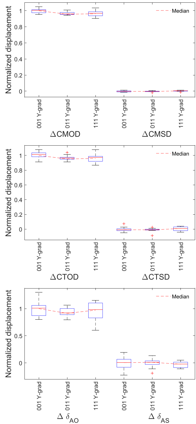
FIGURE 16 Boxplots summarizing normalized distributions of peak \Delta\text{CMD} , \Delta\text{CTD} , and \Delta\delta_A values for multiple texture gradients along Y axis and mean grain size of 5\ \mu\text{m} under force control. The normalization factor is the corresponding opening displacement for [001] orientation [Colour figure can be viewed at wileyonlinelibrary.com ]
