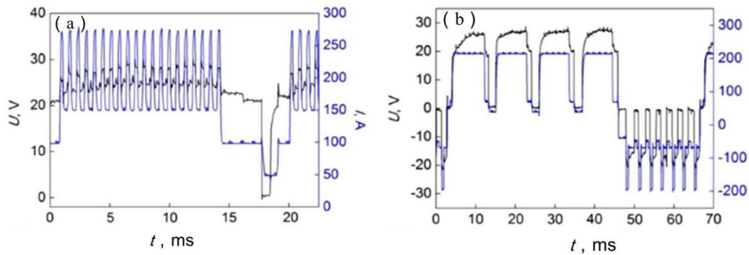
Figure 2. Actual arc current and voltage waveforms of (a) CMT-P and (b) CMT-ADV.
