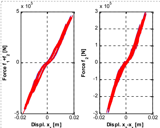
Figure 10. Phase plot of displacements vs. hysteretic force. Simulated in blue, identified in red.
