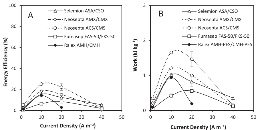
Fig. 3. (A) Energy efficiency obtained and (B) work produced using commercially available membranes in recycle at a range of current densities using a 10 \text{ cm} \times 10 \text{ cm} 5-cell pair RED stack and an intermembrane distance of 0.3 mm. Dilute feed, 0.25 kg 0.02 M; concentrated feed, 0.25 kg 4 M; flow rate, 0.2 \text{ L min}^{-1} . Error bars represent the standard deviation of a triplicate.
