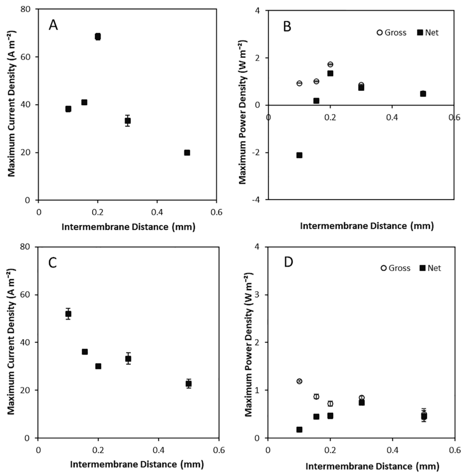
Fig. 5. Spacer thickness in single pass on (A) maximum current and (B) maximum power density at a constant flow rate of 0.2 \text{ L min}^{-1} and (C) maximum current and (D) maximum power density at constant velocity of 0.22 \text{ cm s}^{-1} using a 10 \text{ cm} \times 10 \text{ cm} RED stack containing 5 pairs Neosepta AMX/CMX membranes. Dilute feed, 0.25 \text{ kg } 0.02 \text{ M} ; concentrated feed, 0.25 \text{ kg } 4 \text{ M} ; current, 100 \text{ mA} . Error bars represent the standard deviation of a triplicate.
