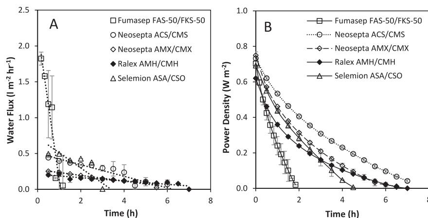
Fig. 4. (A) Water flux and (B) gross power density over time using commercially available membranes in recycle in a 10 \text{ cm} \times 10 \text{ cm} 5-cell pair RED stack with an intermembrane distance of 0.3 \text{ mm} . Dilute feed, 0.25 \text{ kg } 0.02 \text{ M} ; concentrated feed, 0.25 \text{ kg } 4 \text{ M} ; flow rate, 0.2 \text{ L min}^{-1} , current density 10 \text{ A m}^{-2} . Error bars represent the standard deviation of a triplicate.
