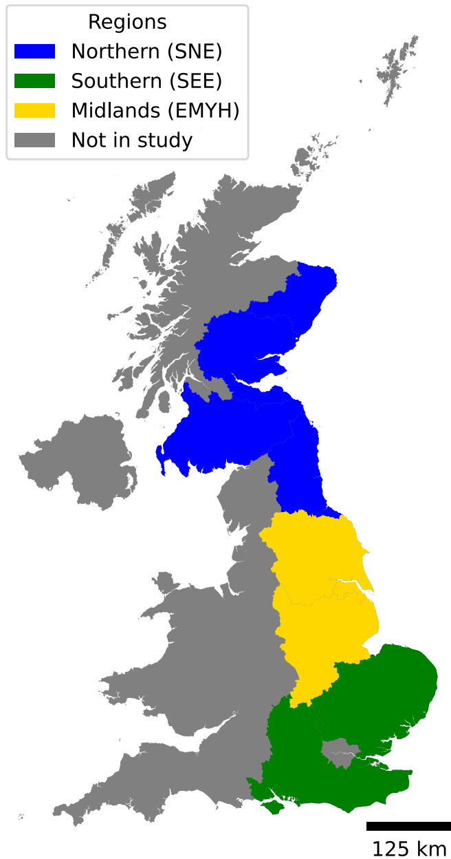
Fig. 2. The three areas of interest for this study. They are formed of the Nuts (European Union, 2024) regions: Northern, SNE (blue): “North Eastern Scotland”, “Eastern Scotland”, “Southern Scotland”, and “North East (England)”, Midlands, EMYH (yellow): “Yorkshire” and “East Midlands (England)”, and Southern SEE (green): “East of England”, “South East (England)”.
