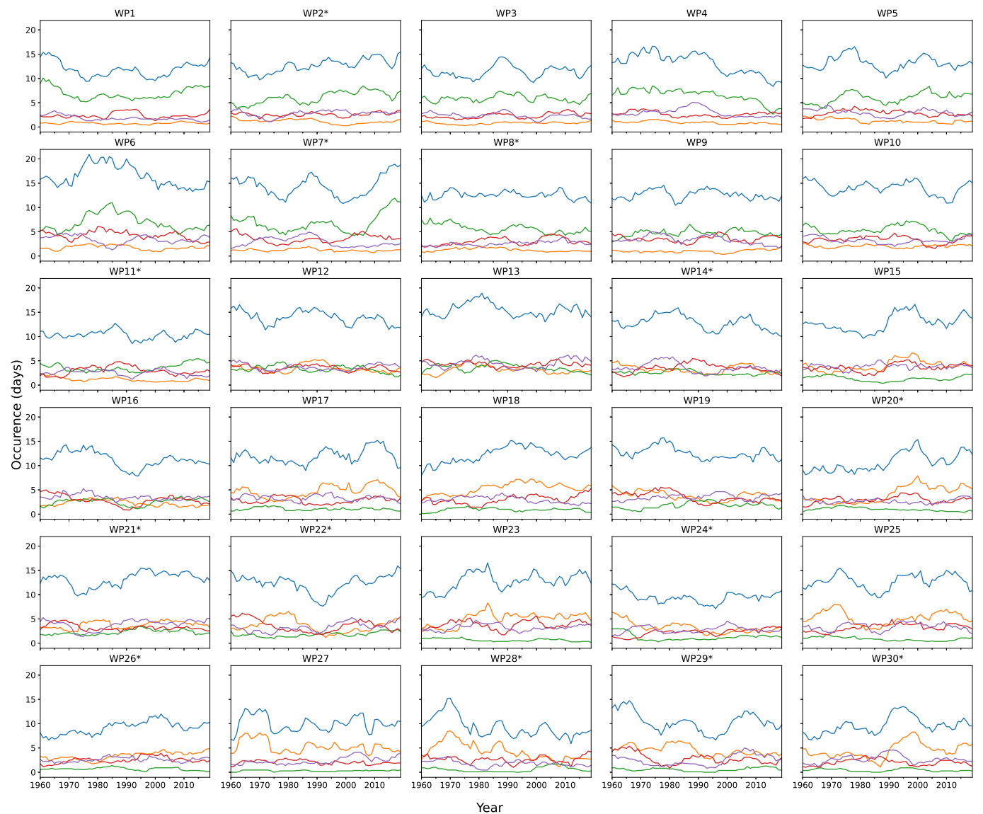
Fig. 6. Shows the number of days each WP occurred between 1960 and 2020 as a rolling average with a window size of 10 years. There is a pane for each MO30; the Y-axis is the number of days the relevant WP occurred, and individual lines represent the four key phenological phases and full-year occurrences. The blue line is the full-year occurrence, purple Planting occurrences, yellow Growth occurrences, red Heading occurrences, and green Filling occurrences. WP with an asterisk are cyclonic patterns.
