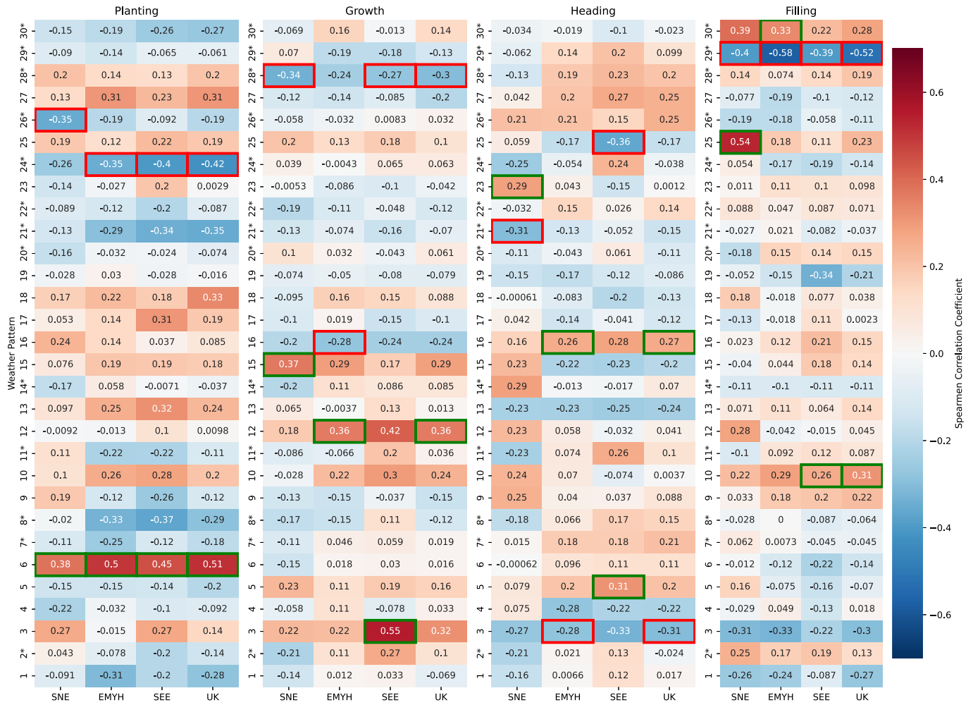
Fig. 5. Spearman correlation between the detrended yield and WP anomalies (1990–2020). Each of the four columns represents the phenological phases (Planting, Growth, Heading, and Filling); in each column, the x-axis shows the three study regions and the entire United Kingdom, while the y-axis indicates each of the 30 WPs. The blue range shows negative correlations, and the red shows positive ones. WPs with an asterisk on the y-axis denote that they are cyclonic. Correlation scores with a green outline indicate the column's (region) maximum value, while red outlines show the minimum. We can see that the cyclonic patterns during Planting correlate to good yield years yet bad yield years during Heading. WP6 during Planting shows a stronger correlation to good yield and WP29 in Filling for bad yield years.
