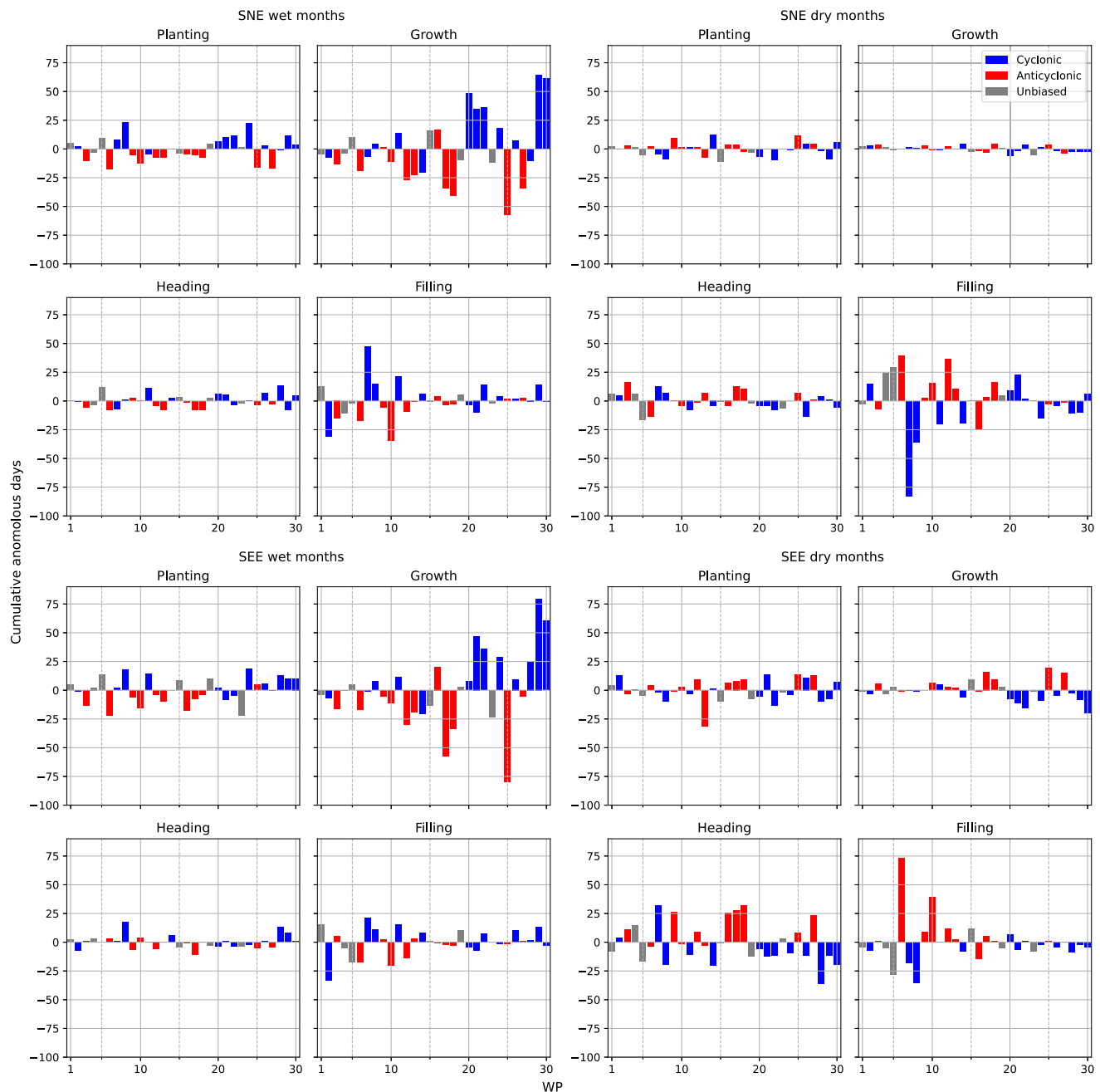
Fig. 3. The accumulated anomalous days when each WP (1–30) was observed during wet ( SPI3 \geq 1 ) and dry ( SPI3 < -1 ) months between 1990 and 2020. Blue bars highlight cyclonic WP, red bars are anticyclonic, and grey are unbiased. The top two rows show the Northern region, and the bottom two are for the Southern (Midlands and Southern are very similar, so Midlands was not included). The left four columns show wet periods, and the right four columns show dry periods. For both wet and dry periods, the data is further broken down into the four key phenological phases, top left of each region's rows and in a clockwise order: Planting, Growth, Heading, and Filling.
