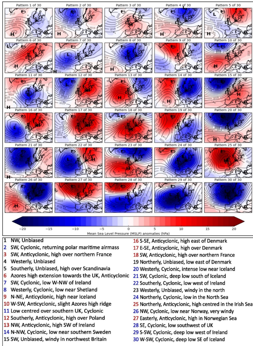
Fig. 1. Definitions for the set of 30 weather patterns (MO30, Mean Sea Level Pressure anomalies, hPa, Neal et al. (2016)). The numbers correspond to each weather pattern's flow over the UK. Numbers in blue represent cyclonic patterns, red indicates anticyclonic patterns, and black signifies unbiased patterns. Abbreviations: NW = northwesterly, S-SE = south-southeasterly, SW = southwesterly, W-SW = west-southwesterly, N-NE = north-northeasterly, E-SE = east-southeasterly.
