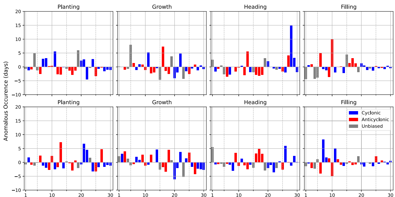
Fig. 7. The number of anomalous days for each WP (the number of days each WP was observed minus the average occurrence over the growing season between 1990 and 2020) for each key phenological phase during the 2012 harvest year (top row, lower than average yield) and 2020 harvest (bottom row, higher than average yield). Blue bars highlight cyclonic WP, red bars are anticyclonic, and grey are unbiased. The columns represent each phenological phase, from left to right: Planting, Growth, Heading, and Filling.
