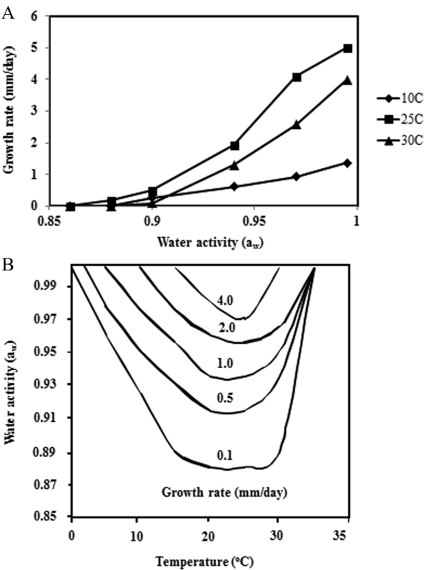
Fig. 3. A, Effect of water activity (a w ) × temperature effects on growth of a strain of Alternaria alternata on a wheat-based medium; B, The growth profile of A. alternata on wheat-based medium showing the optimum and boundary conditions for growth. Numbers on the isopleths join conditions with a similar growth rate (mm/day). Adopted from Magan N and Aldred D [18].
