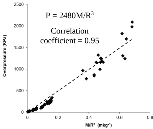
Figure 8. Peak over pressure of the first shock wave in the axial direction plotted against M/R^3 .
