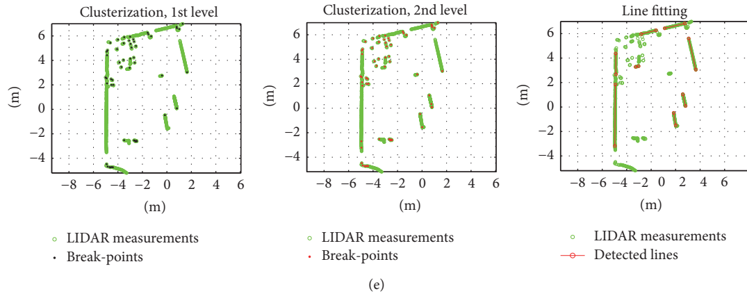
FIGURE 7: From (a) to (e), step-by-step results from the PCA-based line detection algorithm over LIDAR point clouds collected within indoor cluttered areas. (a)-(b) Corridors; (c)-(d)-(e) halls.
