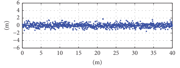
FIGURE 4: Example of simulated point datasets. Setting parameters: m_L = 0 ; n = 1000 ; x_s = 4 cm; \sigma = 50 cm.
