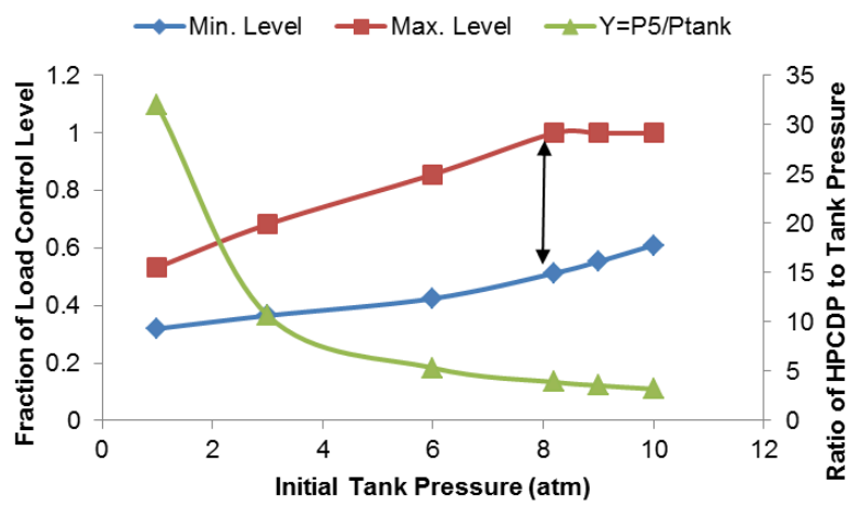
Figure 7: Effect of Tank Pressure on Inventory Control Level
