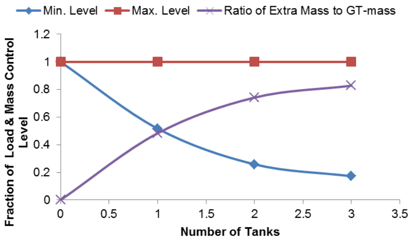
Figure 8: Effect of Number of Tanks
