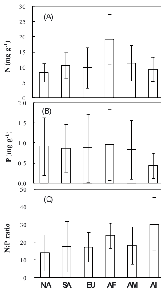
Figure 3. Leaf-litter N concentration (A), P concentration (B) and N:P ratio (C) for flora in North America (NA) ( n = 116 for nitrogen and 97 for phosphorus and N:P ratio), South America (SA) ( n = 50 for nitrogen, 19 for phosphorus and N:P ratio), Europe (EU) ( n = 189 for nitrogen, 113 for phosphorus and N:P ratio), Africa (AF) ( n = 21 for nitrogen, phosphorus and N:P ratio), Asian mainland (AM) ( n = 127 for nitrogen, 103 for phosphorus and N:P ratio) and Asian Islands (AI) ( n = 45 for nitrogen, 33 for phosphorus and N:P ratio). Vertical bars indicate standard deviation. Significant differences between the continents and islands are seen in Table II.
