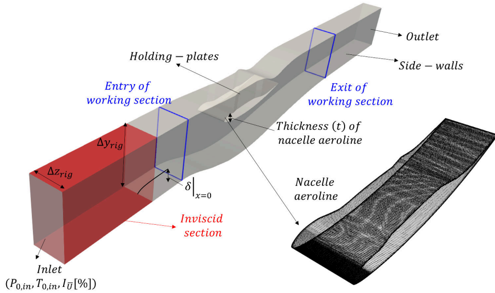
Fig. 2 Schematic of the CFD domain and grid refinement on the nacelle aeroline
