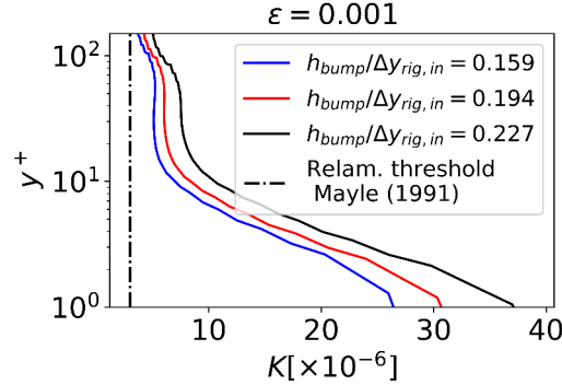
Fig. 13 Boundary layer acceleration on the nacelle aeroline at \Delta z = 0 ahead of the shock ( \Delta x/L_{nac} \approx 0.015 ). M_{in} = 0.65 ; RANS computations with k\omega - SST
