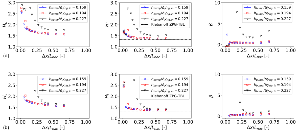
Fig. 18 Boundary layer characteristics on the nacelle aeroline at \Delta z = 0 . RANS with a) k\omega - SST and b) \gamma - Re_\theta turbulence models
