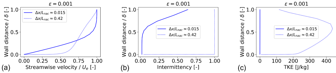
Fig. 19 a) Non-dimensional streamwise velocity, b) intermittency and c) turbulent kinetic energy distributions across the boundary layer on the nacelle aeroline at \Delta z = 0 . h_{bump}/\Delta y_{rig,in} = 0.227 . RANS with \gamma - Re_\theta turbulence model
