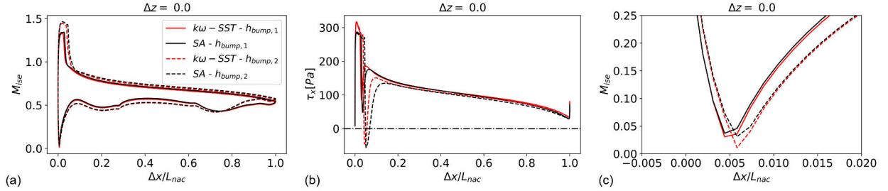
Fig. 6 Effect of turbulence model on a) M_{ise} , b) \tau_x distributions and c) position of the stagnation point on the nacelle cowl at \Delta z = 0
