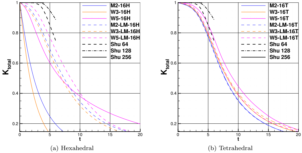
Figure 23: Total kinetic energy K temporal evolution for various schemes, and LM treatment for the 3D Taylor-Green vortex test problem at the coarse grid resolutions, and comparison with the WENO obtained solutions of [70].
